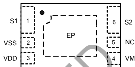
U-DFN2535-6 (Type B) (Option 1)
