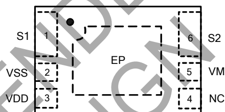
U-DFN2535-6 (Type B) (Option 2)
