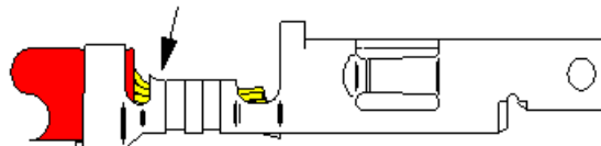
Good Crimp
