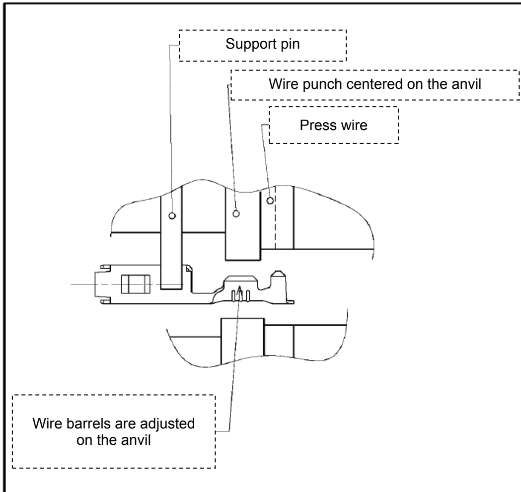
Figure 6a – TERMINAL POSITION IN TOOL
