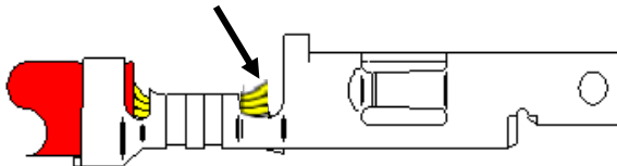
Bad Crimp
