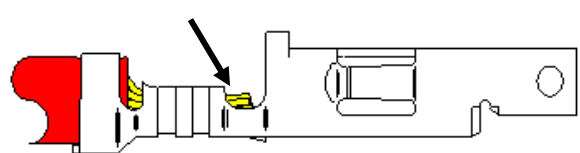
Good Crimp
