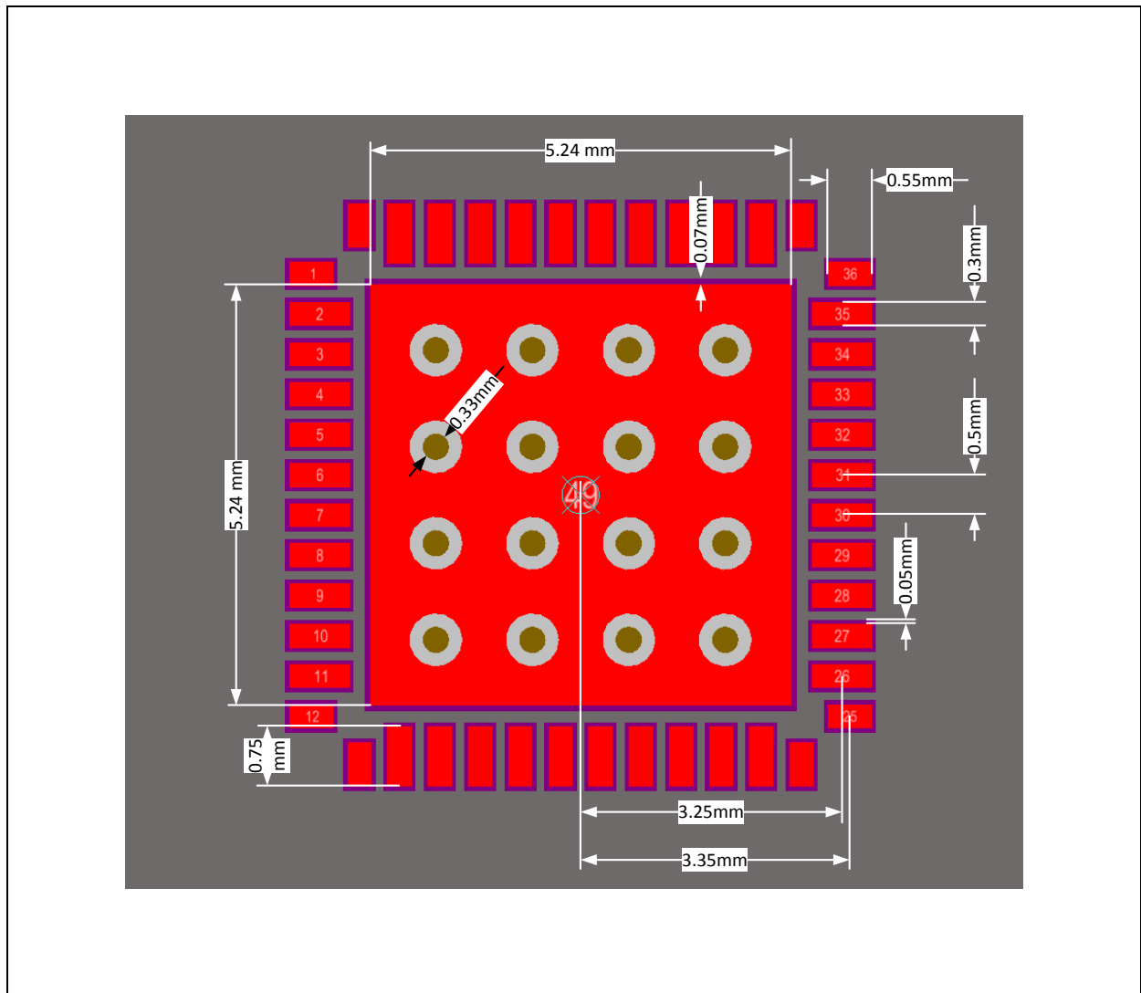
Figure 8: Recommended PCB Pad Layout
