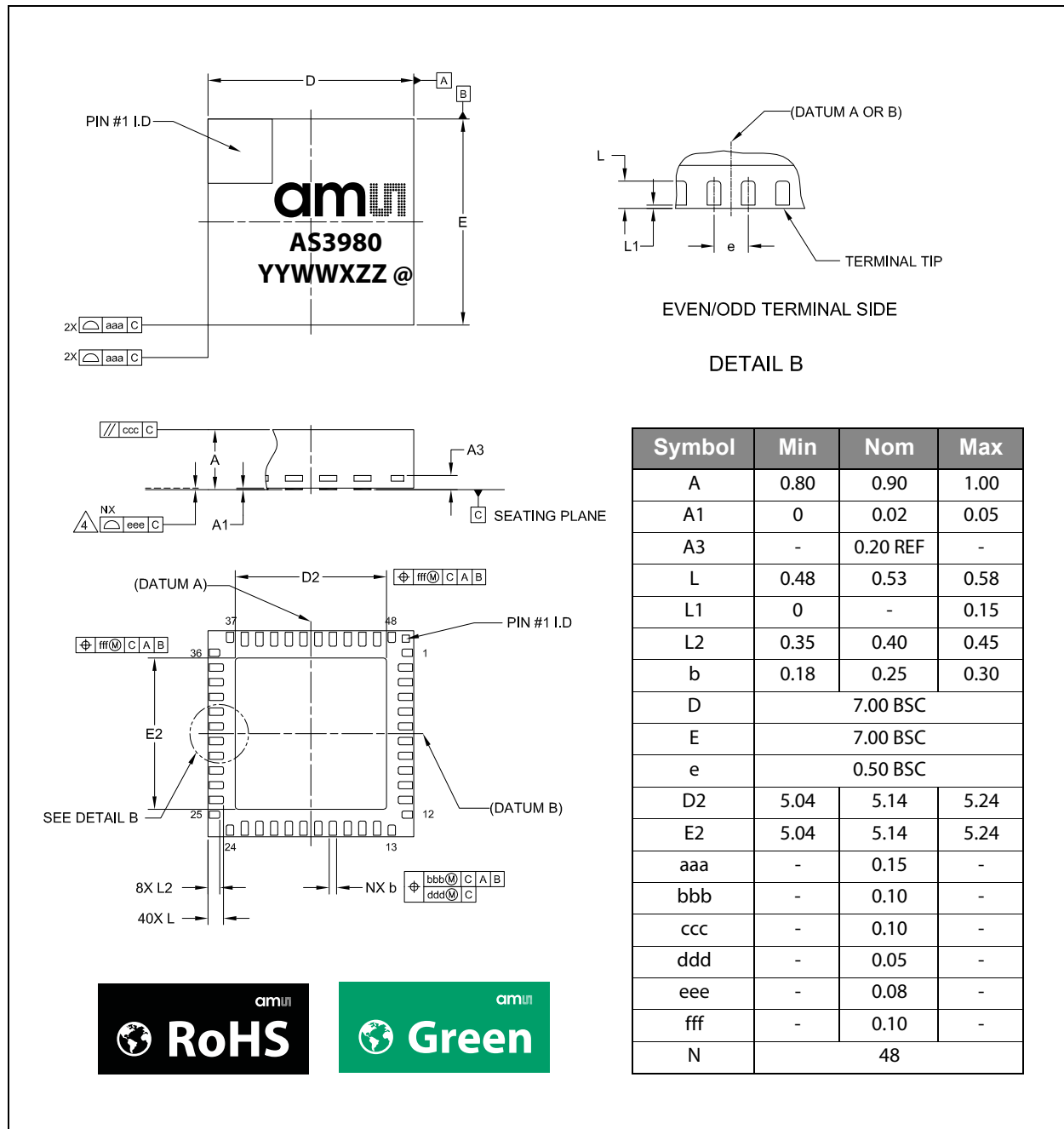
Figure 13: Package Drawings
