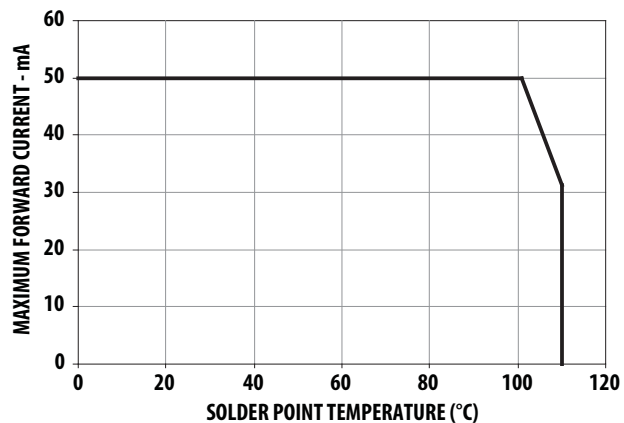
Figure 4b. Maximum forward current vs. solder point temperature. Derated Based on T_{JMAX} = 125^{\circ}\text{C} , R\theta_{JP} = 110^{\circ}\text{C/W}
