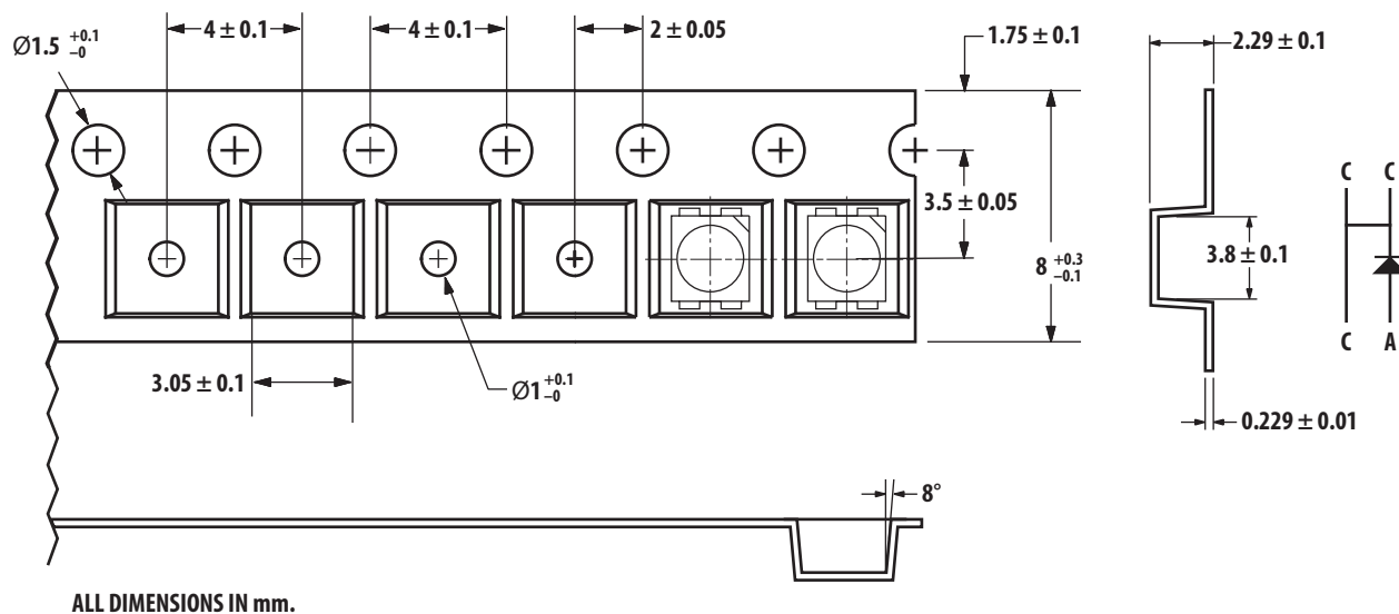
Figure 10. Tape Dimensions
