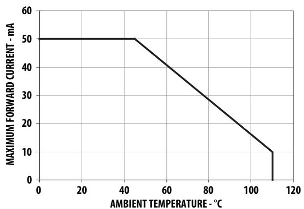
Figure 4a. Maximum Forward Current Vs. Ambient Temperature. Derated Based on T_{JMAX} = 125^{\circ}\text{C} , R\theta_{JA} = 300^{\circ}\text{C/W}
