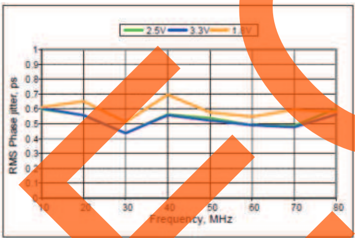
1MHz-80MHz Devices
