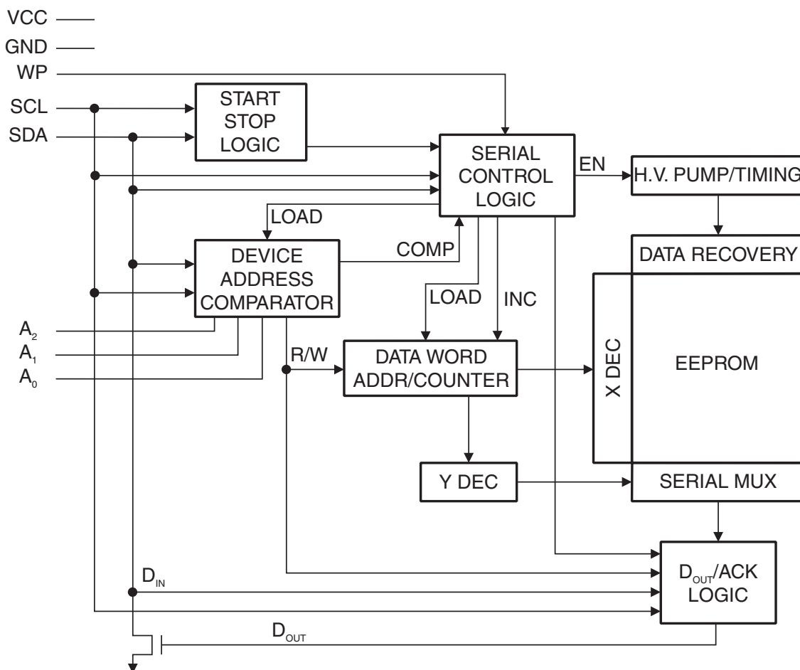
Figure 0-1. Block Diagram
