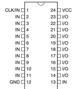
Figure 2-2. DIP/SOIC
