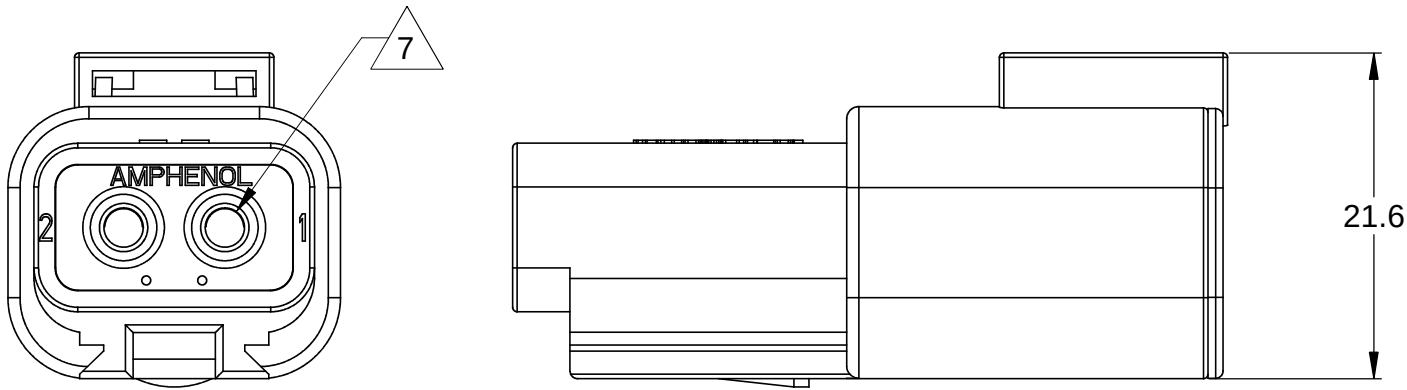
REFERENCE DIMENSIONS - ASSEMBLED RECEPTACLE
