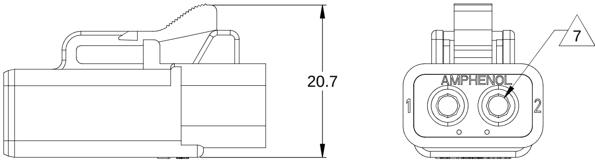
REFERENCE DIMENSIONS - ASSEMBLED PLUG
