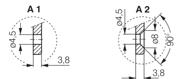
Barbed inserts
