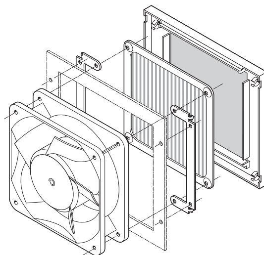
LZ60 Filter
