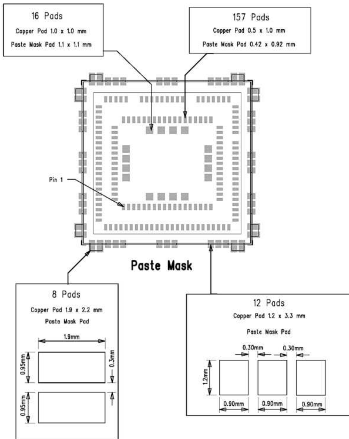
Figure 13. Recommended WP and RC76 Series Snap-in Socket Footprint – Paste Mask Layout
