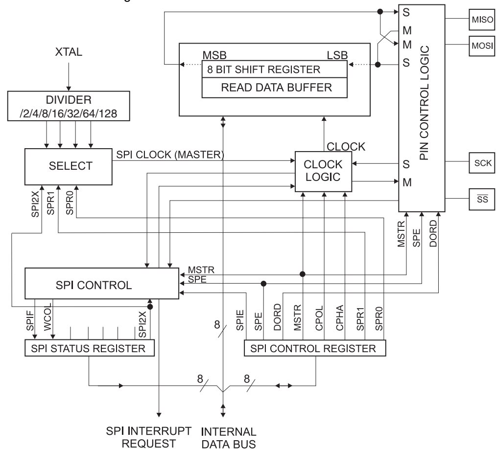
Figure 57. SPI Block Diagram (1)
