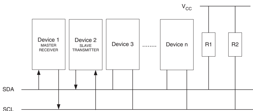
Figure 80. Data Transfer in Master Receiver Mode
