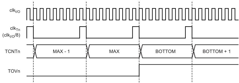
Figure 10-9. Timer/Counter Timing Diagram, with Prescaler ( f_{\text{clk}_{I/O}}/8 )
