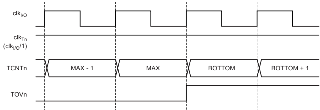
Figure 10-8. Timer/Counter Timing Diagram, no Prescaling
