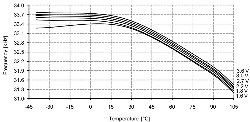
Figure 33-228. Ultra Low-Power Internal Oscillator Frequency vs. Temperature
