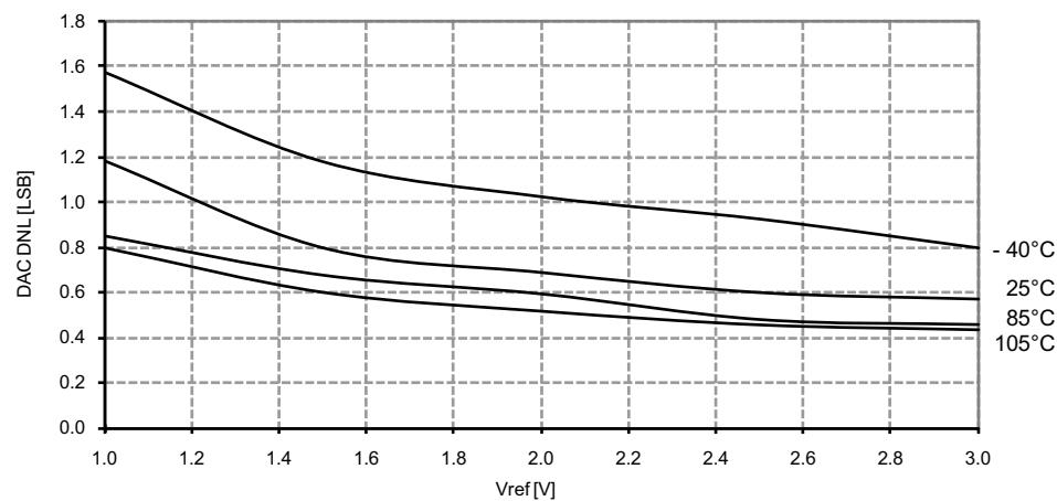
Figure 33-208. DNL Error vs. V_{REF} V_{CC} = 3.6V
