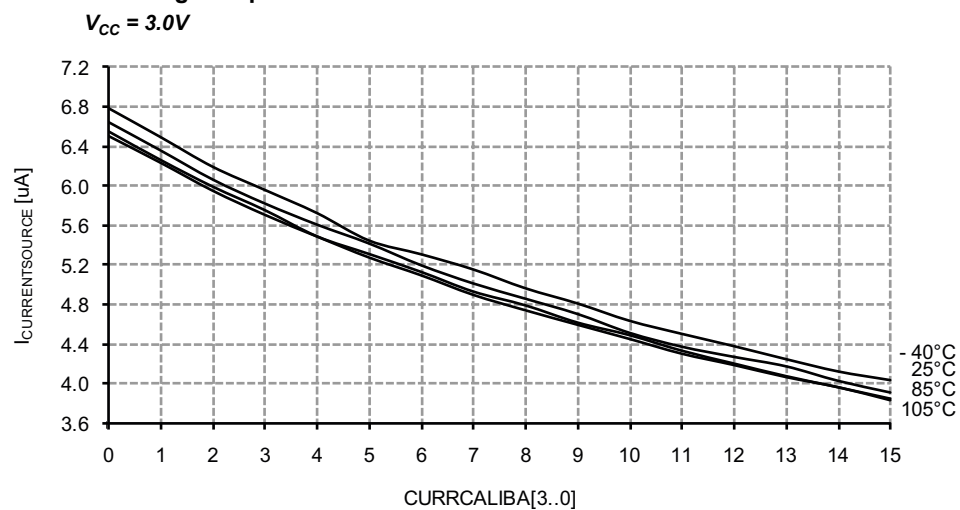
Figure 33-215. Analog Comparator Current Source vs. Calibration Value
