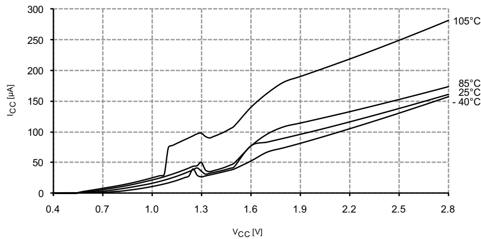
Figure 33-227. Power-on Reset Current Consumption vs. V_{CC} BOD level = 3.0V, enabled in sampled mode
