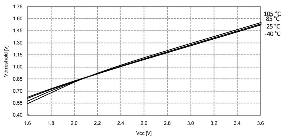
Figure 33-276. I/O Pin Input Threshold Voltage vs. V_{CC}
