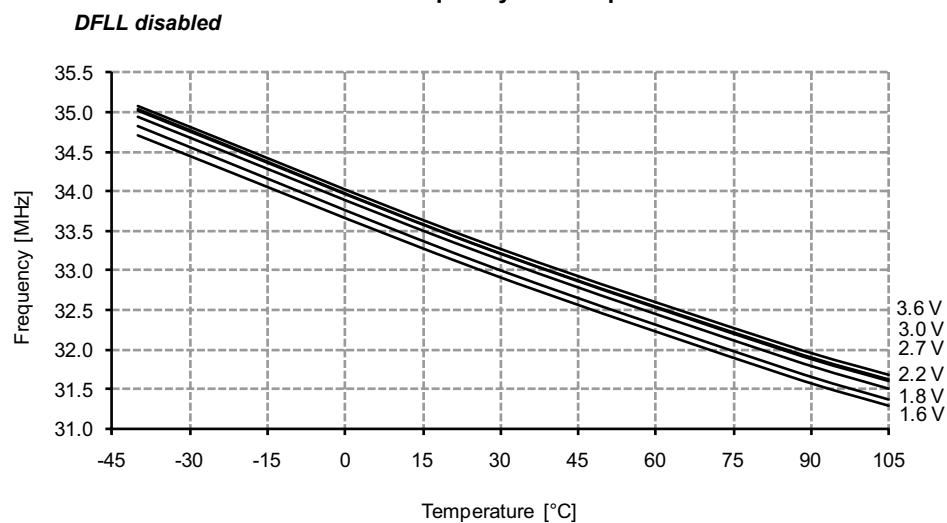
Figure 33-234. 32MHz Internal Oscillator Frequency vs. Temperature
