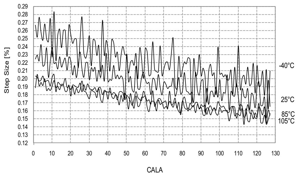
Figure 33-70. 2MHz Internal Oscillator CALA Calibration Step Size V_{CC} = 3V
