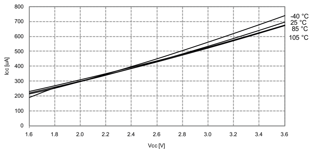
Figure 33-246. Active Mode Supply Current vs. V_{CC}
