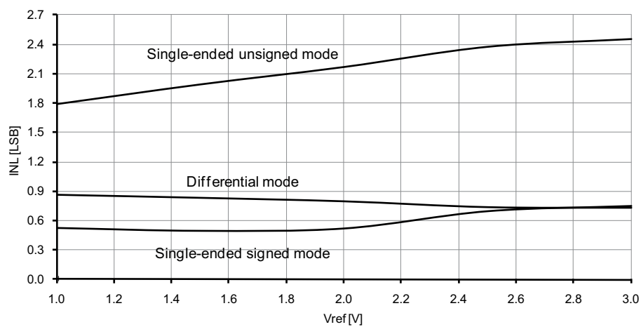
Figure 33-194. INL Error vs. External V_{REF} T = 25^\circ\text{C} , V_{CC} = 3.6\text{V} , external reference
