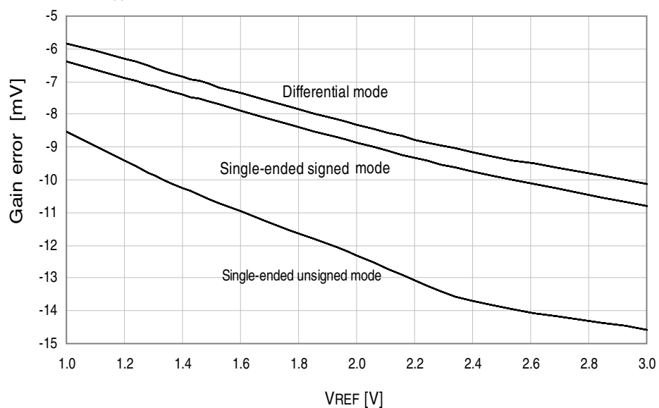
Figure 33-42. Gain Error vs. V_{REF}
