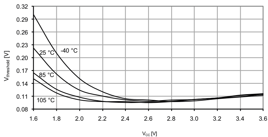
Figure 33-193. I/O Pin Input Hysteresis vs. V_{CC}
