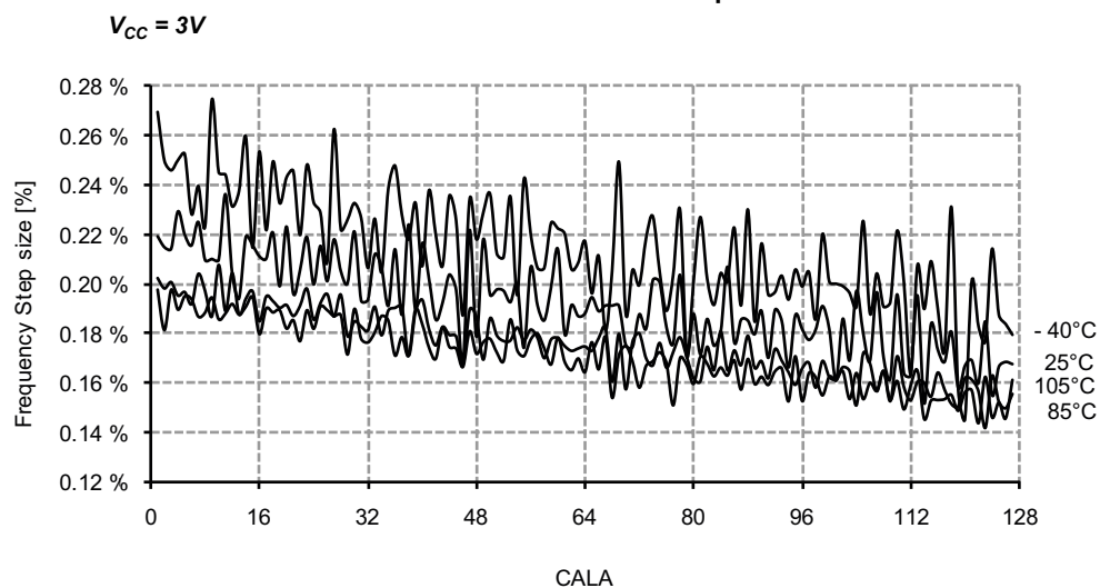
Figure 33-233. 2MHz Internal Oscillator CALA Calibration Step Size
