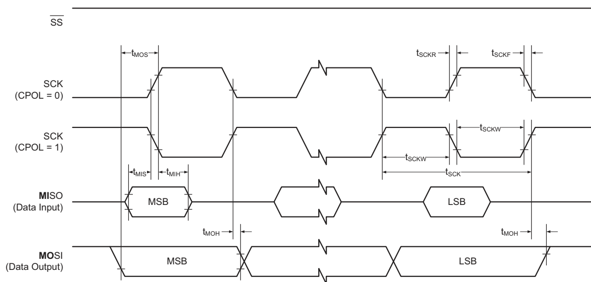
Figure 32-5. SPI Timing Requirements in Master Mode
