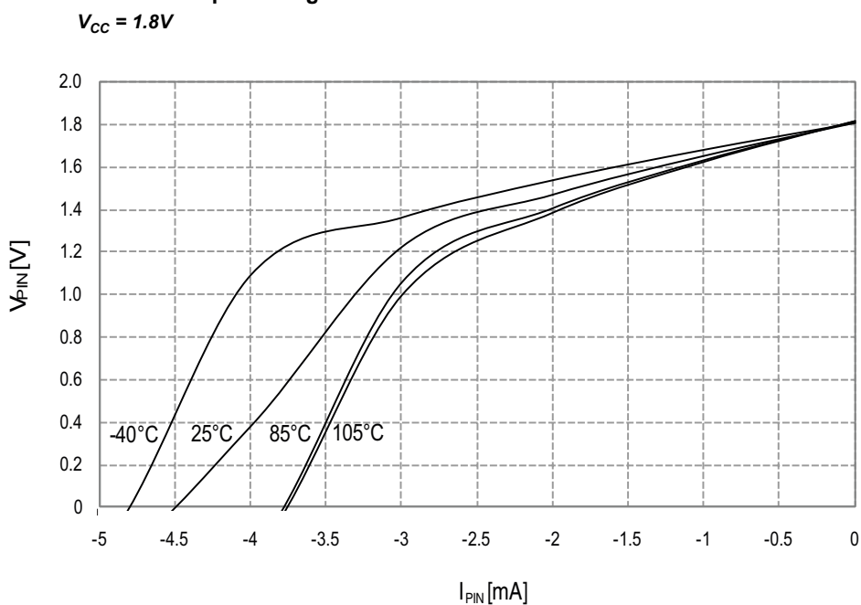
Figure 33-103. I/O Pin Output Voltage vs. Source Current
