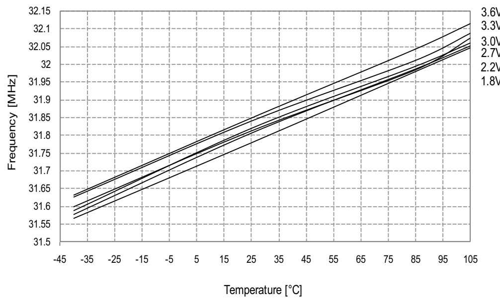
Figure 33-151. 32MHz Internal Oscillator Frequency vs. Temperature DPLL enabled, from the 32.768kHz internal oscillator
