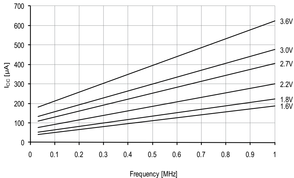
Figure 33-160. Active Supply Current vs. Frequency
