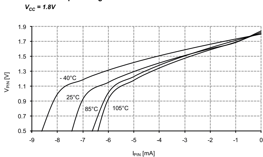
Figure 33-182. I/O Pin Output Voltage vs. Source Current
