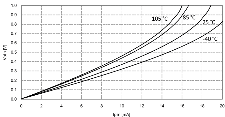
Figure 33-270. I/O Pin Output Voltage vs. Sink Current V_{CC} = 1.8V
