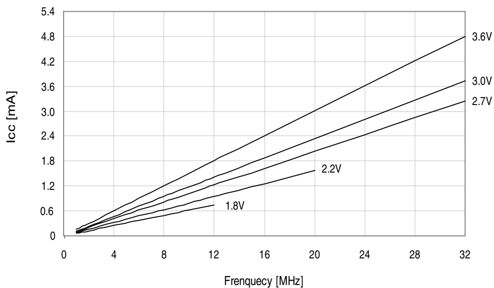
Figure 33-251. Idle Mode Supply Current vs. Frequency
