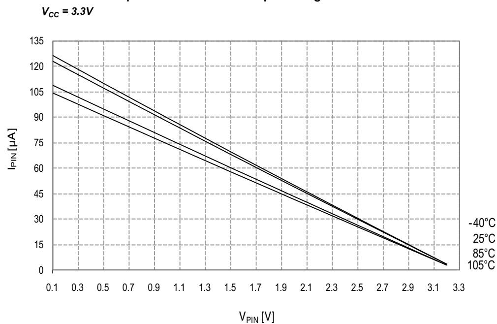
Figure 33-102. I/O Pin Pull-up Resistor Current vs. Input Voltage
