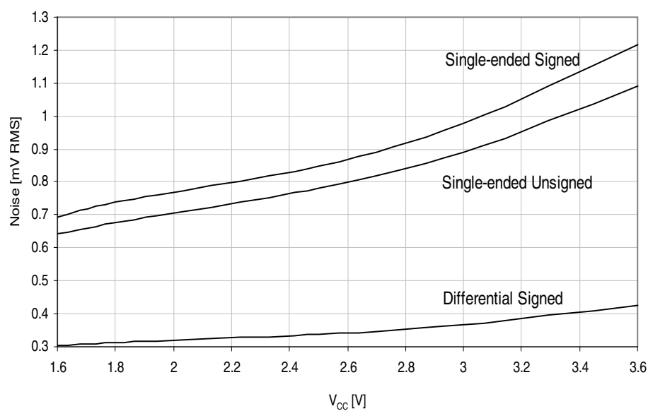
Figure 33-290. Noise vs. V_{CC}
