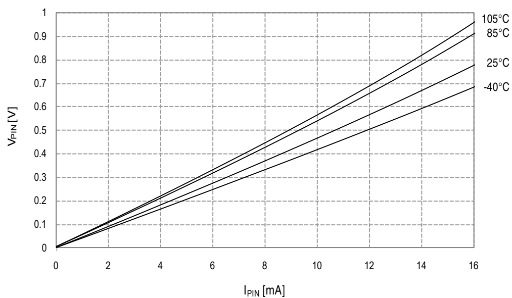
Figure 33-30. I/O Pin Output Voltage vs. Sink Current
