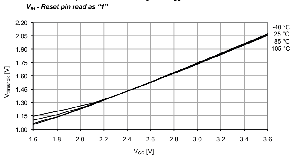
Figure 33-308. Reset Pin Input Threshold Voltage vs. V_{CC}
