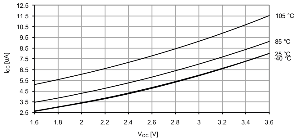
Figure 33-177. Standby Supply Current vs. V_{CC} Standby, f_{SYS} = 1\text{MHz}
