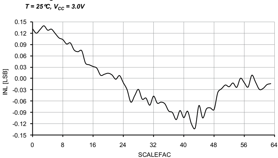
Figure 33-216. Voltage Scaler INL vs. SCALEFAC
