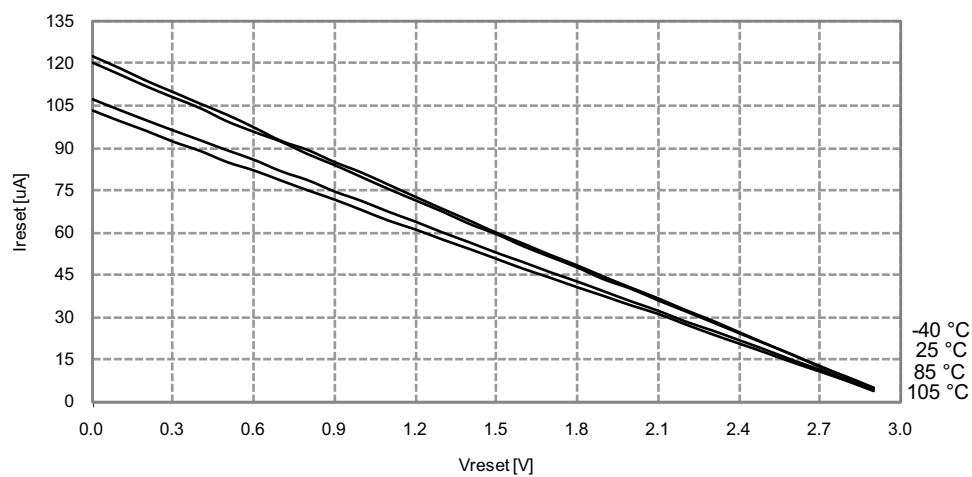
Figure 33-306. Reset Pin Pull-up Resistor Current vs. Reset Pin Voltage
