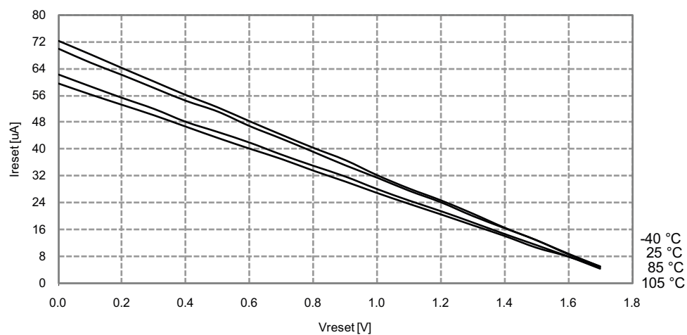
Figure 33-305. Reset Pin Pull-up Resistor Current vs. Reset Pin Voltage
