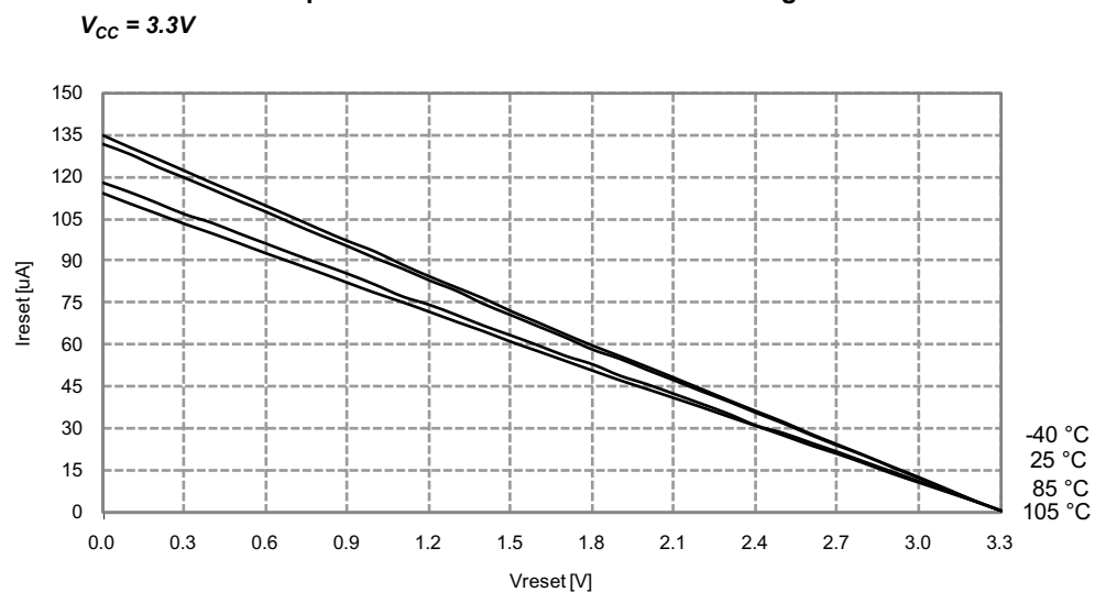
Figure 33-307. Reset Pin Pull-up Resistor Current vs. Reset Pin Voltage
