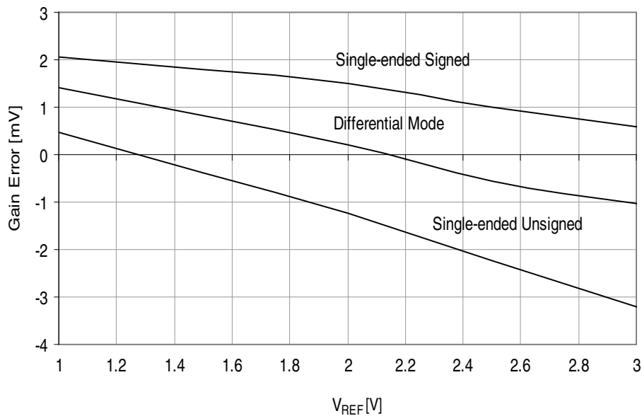
Figure 33-284. Gain Error vs. V_{REF} T = 25^{\circ}\text{C} , V_{CC} = 3.6\text{V} , ADC sampling speed = 500ksps
