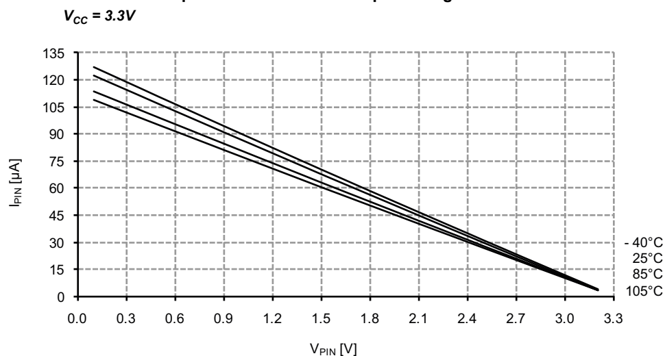
Figure 33-181. I/O Pin Pull-up Resistor Current vs. Input Voltage
