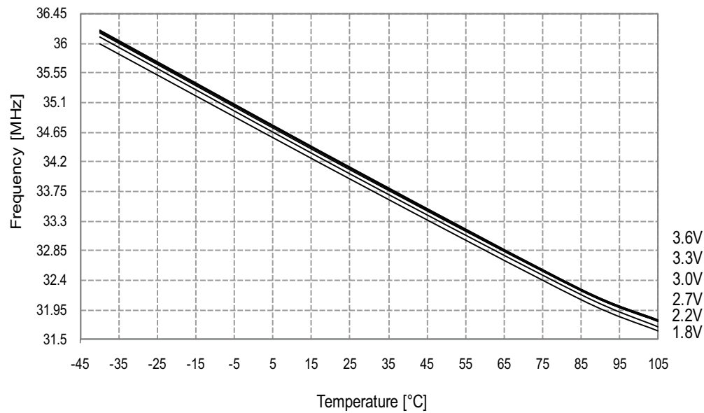
Figure 33-150. 32MHz Internal Oscillator Frequency vs. Temperature DPLL disabled
