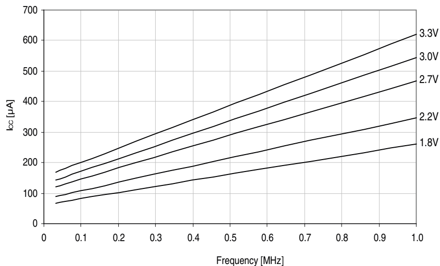
Figure 33-2. Active Supply Current vs. Frequency
