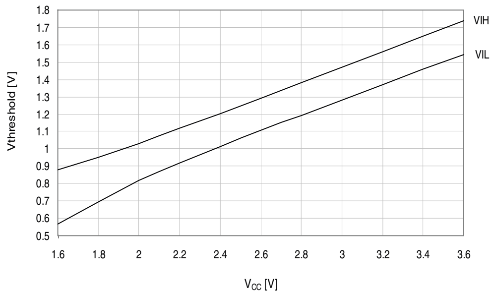
Figure 33-111. I/O Pin Input Threshold Voltage vs. V_{CC}
