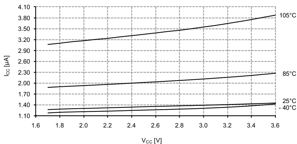
Figure 33-175. Power-down Mode Supply Current vs. V_{CC} Watchdog and sampled BOD enabled
