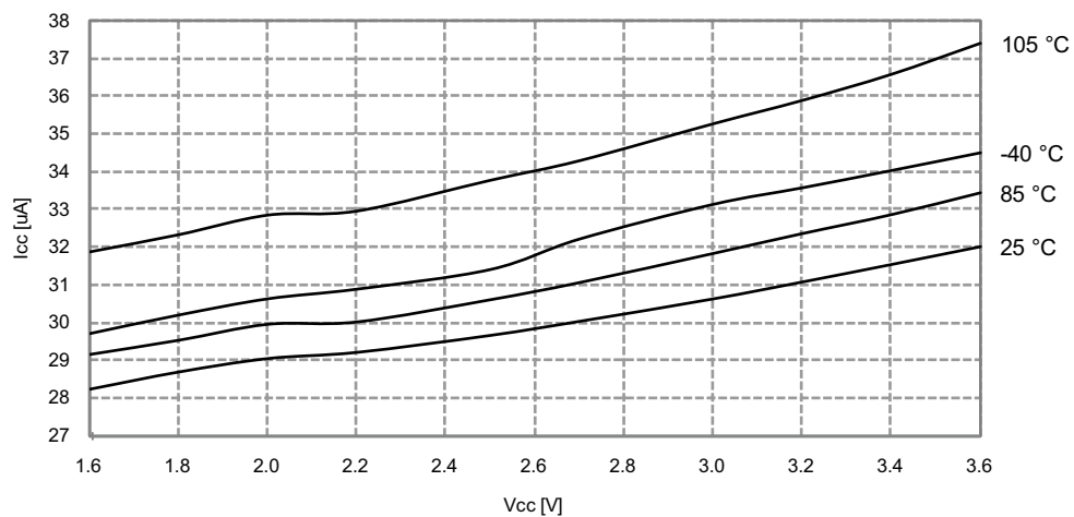
Figure 33-252. Idle Mode Supply Current vs. V CC
