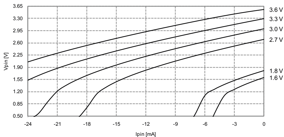
Figure 33-269. I/O Pin Output Voltage vs. Source Current
