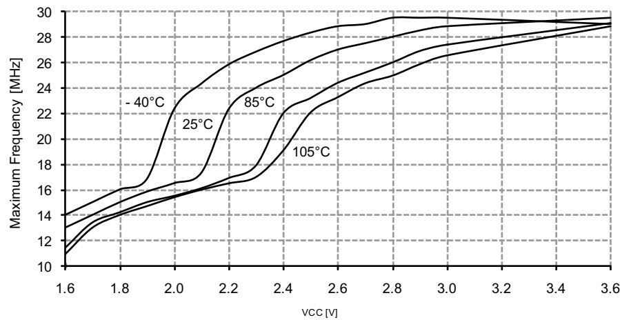
Figure 33-242. Maximum PDI Frequency vs. V_{CC}
