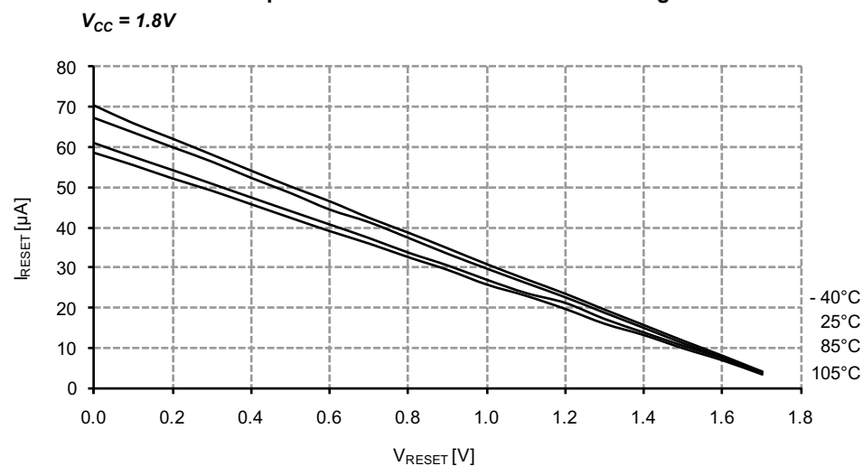
Figure 33-221. Reset Pin Pull-up Resistor Current vs. Reset Pin Voltage
