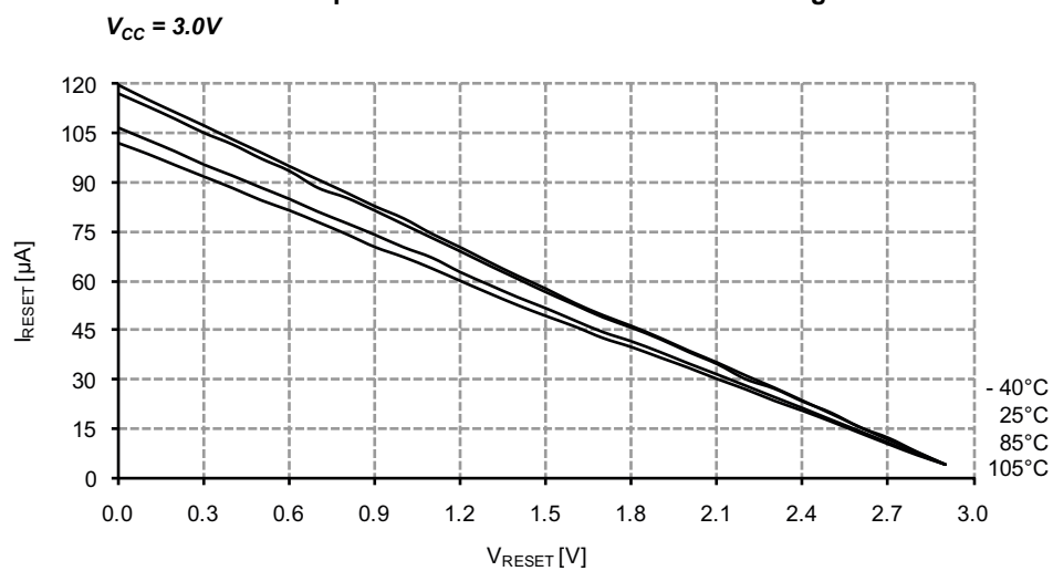
Figure 33-222. Reset Pin Pull-up Resistor Current vs. Reset Pin Voltage
