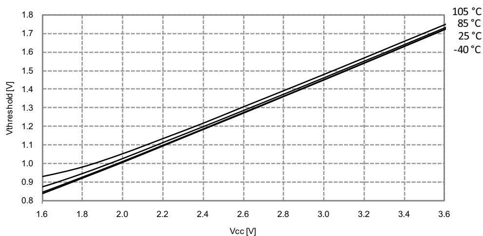
Figure 33-275. I/O Pin Input Threshold Voltage vs. V_{CC}
