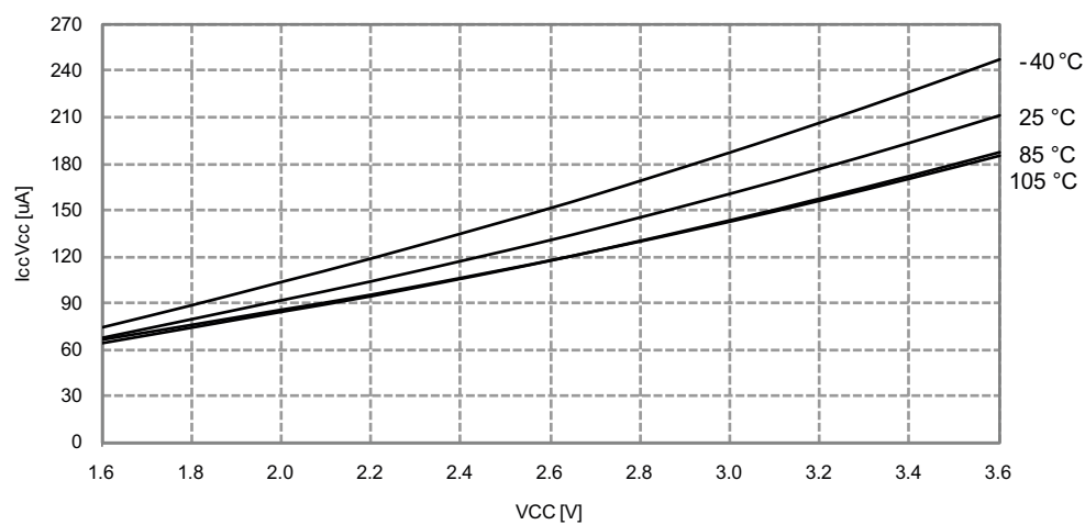
Figure 33-245. Active Mode Supply Current vs. V_{CC}
