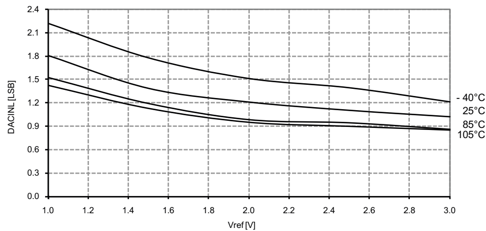
Figure 33-207. DAC INL Error vs. V_{REF} V_{CC} = 3.6V
