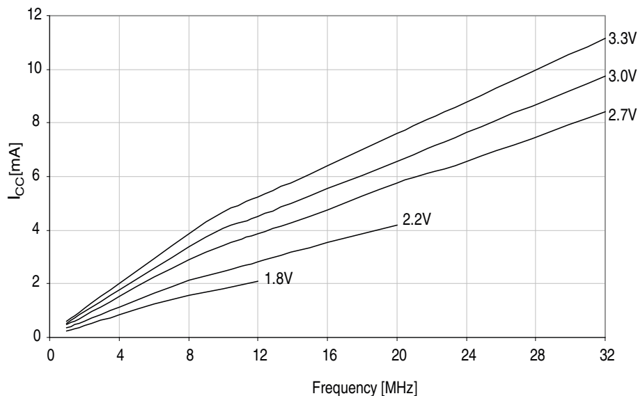
Figure 33-2. Active Supply Current vs. Frequency
