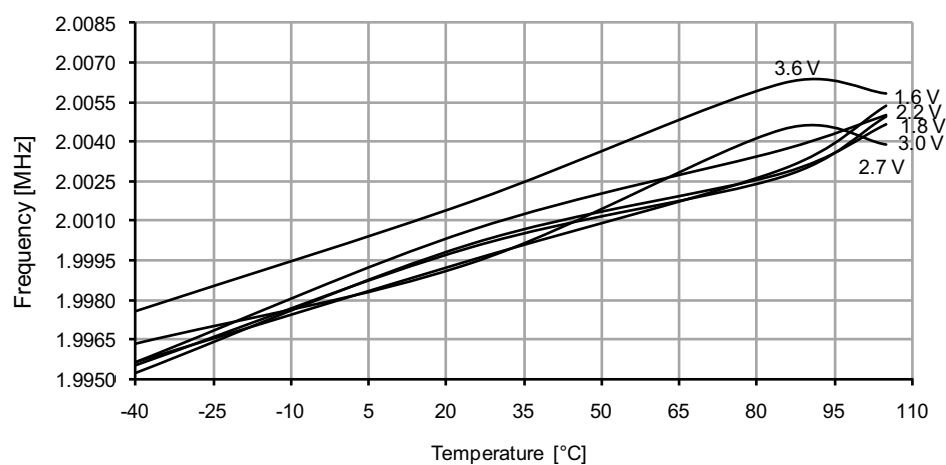
Figure 37-74. 2MHz internal oscillator frequency vs. temperature.
