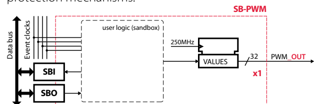
Fig. 18. Internal structure of the SB-PWM block.
