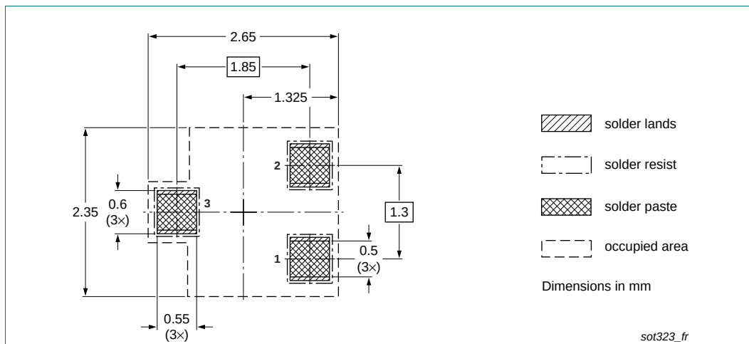
Fig 6. Reflow soldering footprint SOT323 (SC-70)
