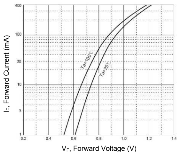
Figure 1. Forward Characteristics
