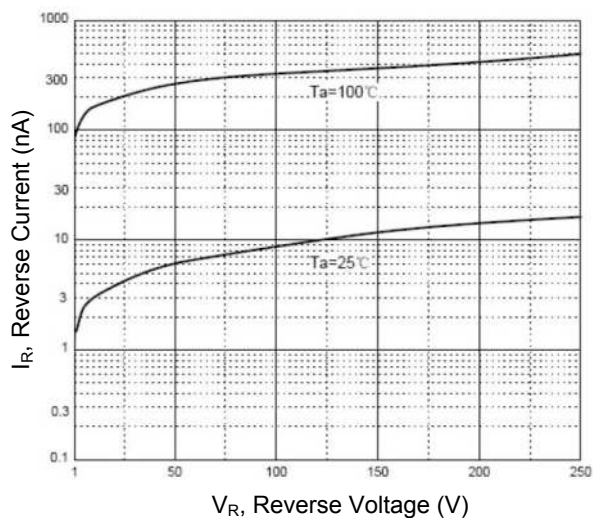
Figure 2. Reverse Characteristics
