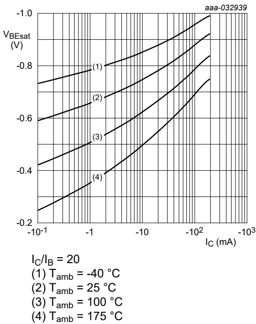
Fig. 14. TR2 (PNP): Base-emitter saturation voltage as a function of collector current; typical values
