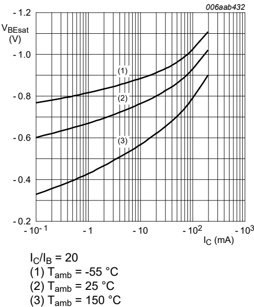
Fig. 7. Per transistor: Base-emitter saturation voltage as a function of collector current; typical values
