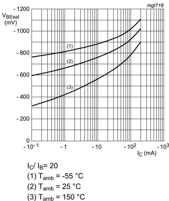
Fig. 11. BC856BQC: Base-emitter saturation voltage as a function of collector current; typical values
