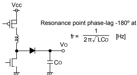
LC Resonance
