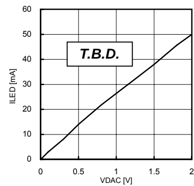
Fig.12 VDAC gain
