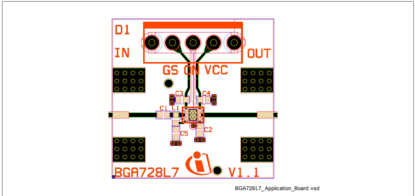
Figure 3 Application Board
