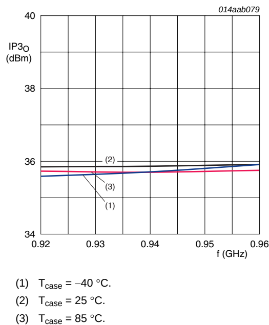
Fig 33. Output third-order intercept point as a function of frequency
