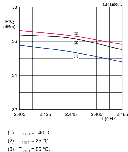
Fig 27. Output third-order intercept point as a function of frequency
