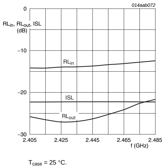
Fig 26. Input return loss, output return loss and isolation as a function of frequency
