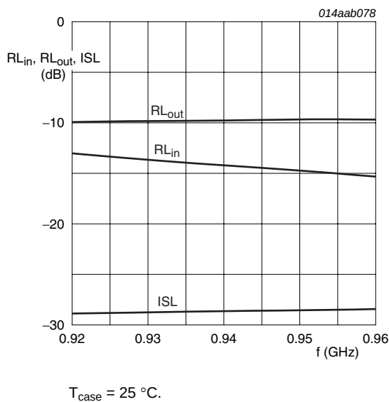
Fig 32. Input return loss, output return loss and isolation as a function of frequency
