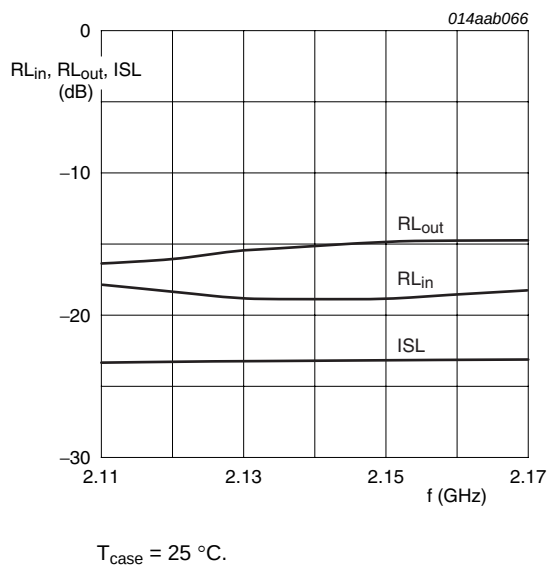
Fig 20. Input return loss, output return loss and isolation as a function of frequency
