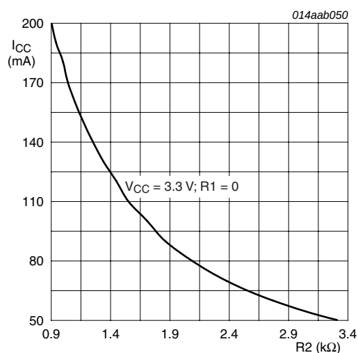
b. 3.3 V supply voltage
