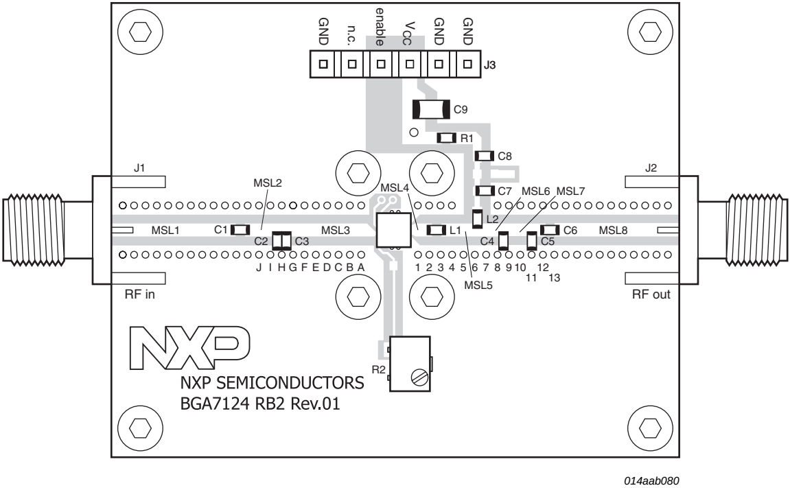
Fig 34. 3.3 V/130 mA application reference board; 920 MHz to 960 MHz
