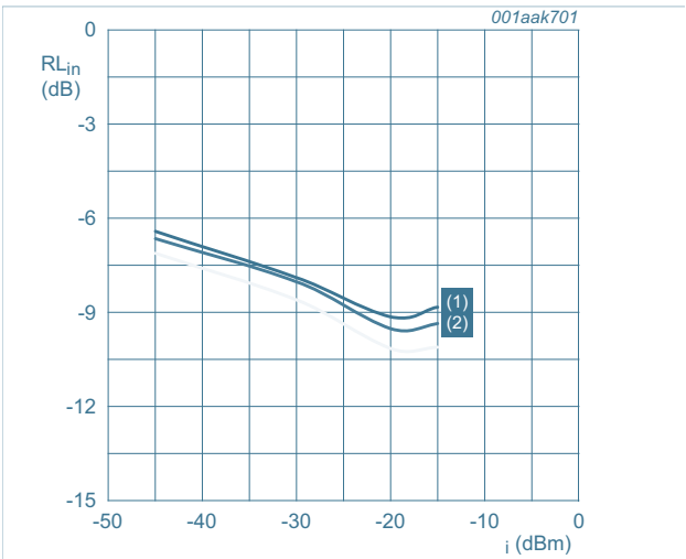
Fig 16. Input return loss as a function of input power; typical values
