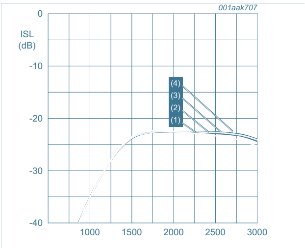
V_{CC} = 1.8\text{ V} ; T_{amb} = 25\text{ }^{\circ}\text{C} . (1) P_i = -45\text{ dBm} (2) P_i = -30\text{ dBm} (3) P_i = -20\text{ dBm} (4) P_i = -15\text{ dBm}
