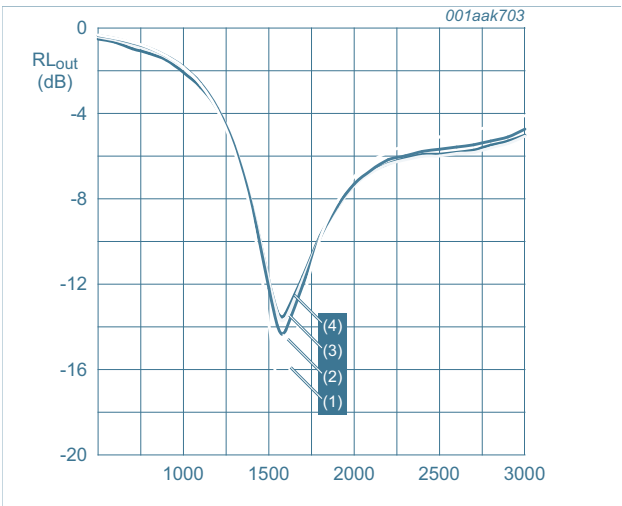
Fig 18. Output return loss as a function of frequency; typical values
