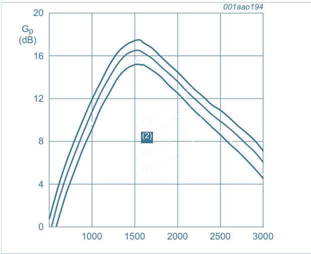
V_{CC} = 1.8\text{ V} ; P_i = -45\text{ dBm} . (1) T_{amb} = -40\text{ }^{\circ}\text{C} (2) T_{amb} = +25\text{ }^{\circ}\text{C} (3) T_{amb} = +85\text{ }^{\circ}\text{C} (4) T_{amb} = +125\text{ }^{\circ}\text{C}
