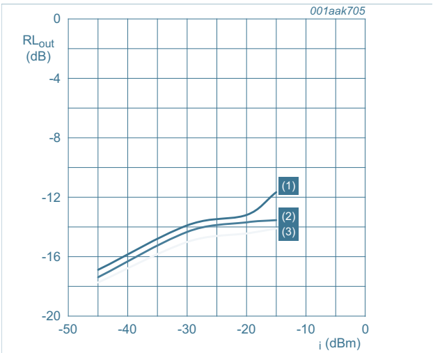
T_{amb} = 25\text{ }^{\circ}\text{C} ; f = 1575\text{ MHz} . (1) V_{CC} = 1.5\text{ V} (2) V_{CC} = 1.8\text{ V} (3) V_{CC} = 2.85\text{ V}
