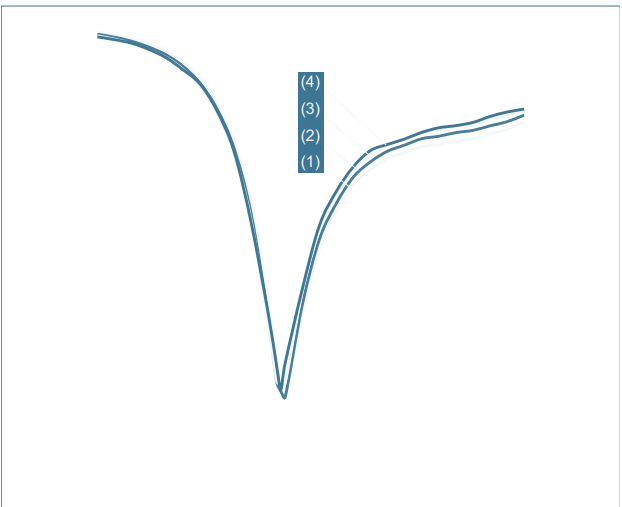
Fig 17. Output return loss as a function of frequency; typical values
