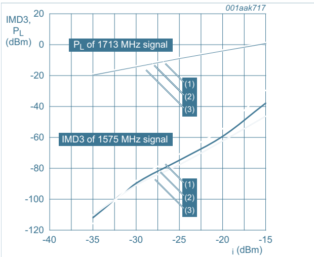
f = 1575 \text{ MHz}; f_1 = 1713 \text{ MHz}; f_2 = 1851 \text{ MHz}; T_{\text{amb}} = 25 \text{ }^{\circ}\text{C}. (1) V_{\text{CC}} = 1.5 \text{ V} (2) V_{\text{CC}} = 1.8 \text{ V} (3) V_{\text{CC}} = 2.85 \text{ V}
