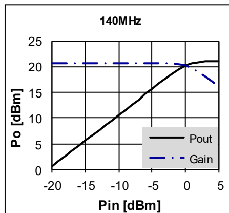
140MHz, 5V/85mA
