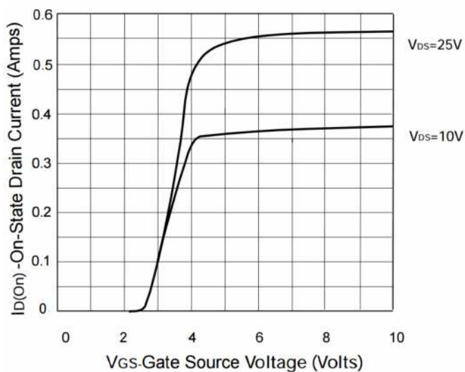
Transfer characteristics
