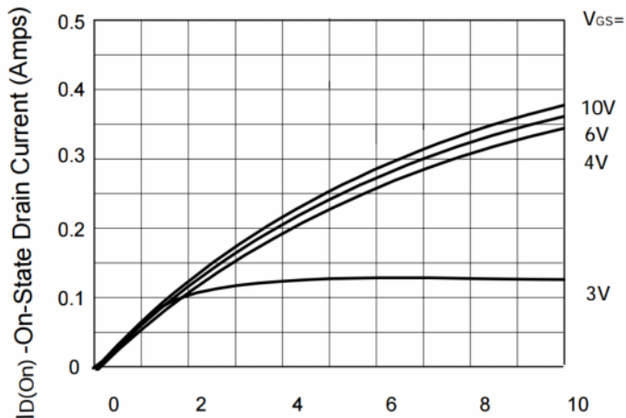
Saturation Characteristics
