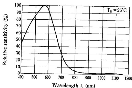
Fig. 4 Spectral Sensitivity
