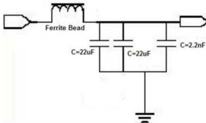
Figure 57. \text{XCOREV}_{\text{DD}} and \text{XPADV}_{\text{DD}} Power Supply Filter Circuit
