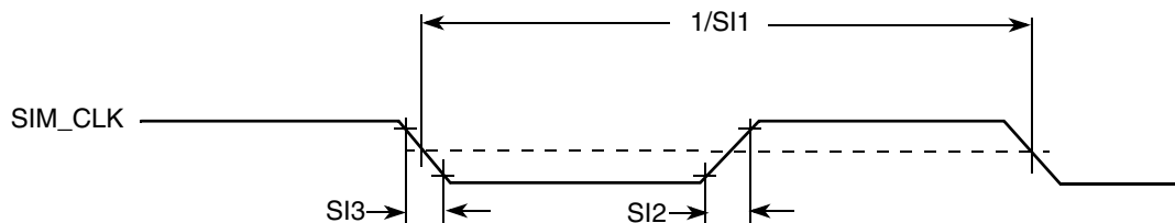
Figure 50. USIM Clock Timing Diagram
