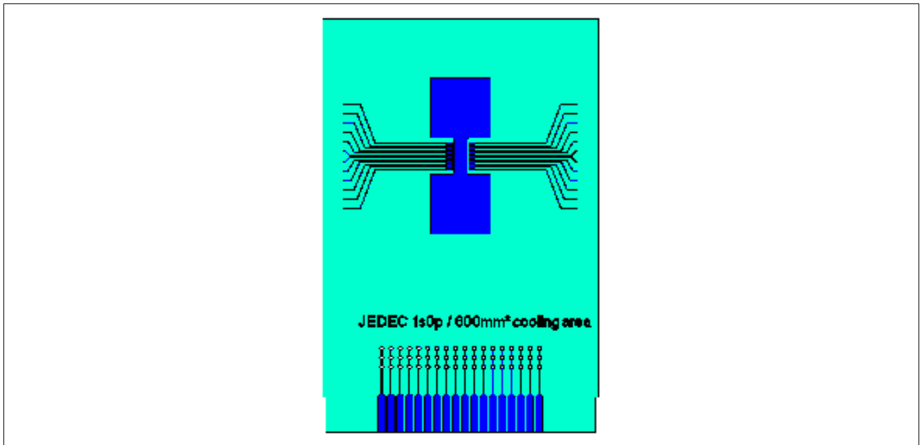
Figure 5 PC Board for Thermal Simulation with 600 mm² Cooling Area
