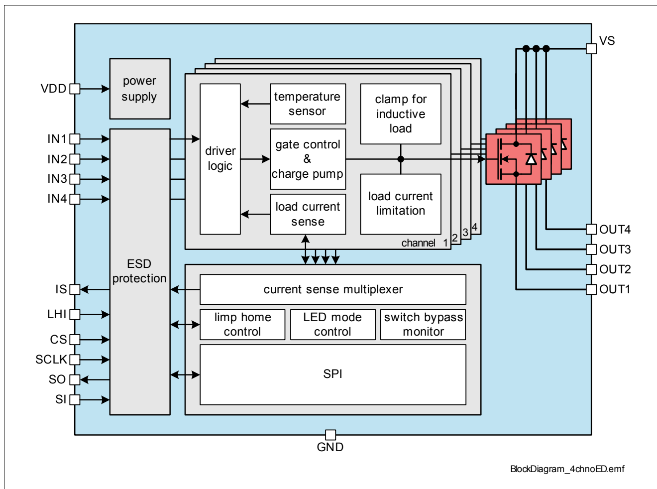
Figure 1 Block Diagram BTS54040-LBA
