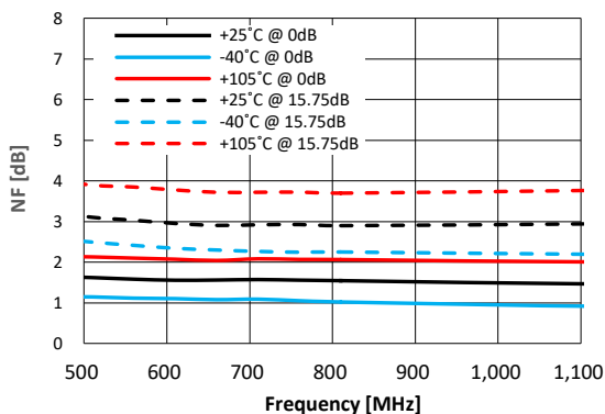
Figure 18. Noise Figure vs. Frequency @ VDD = 5V Over Temperature (Max Gain State)
