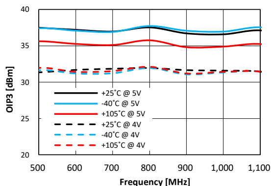
Figure 15. OIP3 vs. Frequency vs. VDD Over Temperature (Max Gain State)
