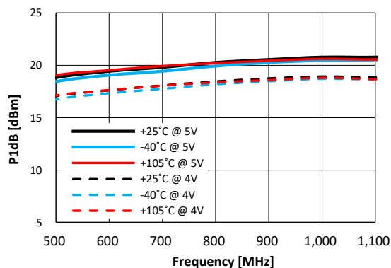
Figure 17. P1dB vs. Frequency vs VDD Over Temperature (Max Gain State)
