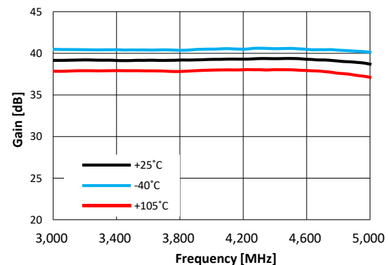
Figure 44. Gain vs. Frequency @ VDD = 4V over Temperature
