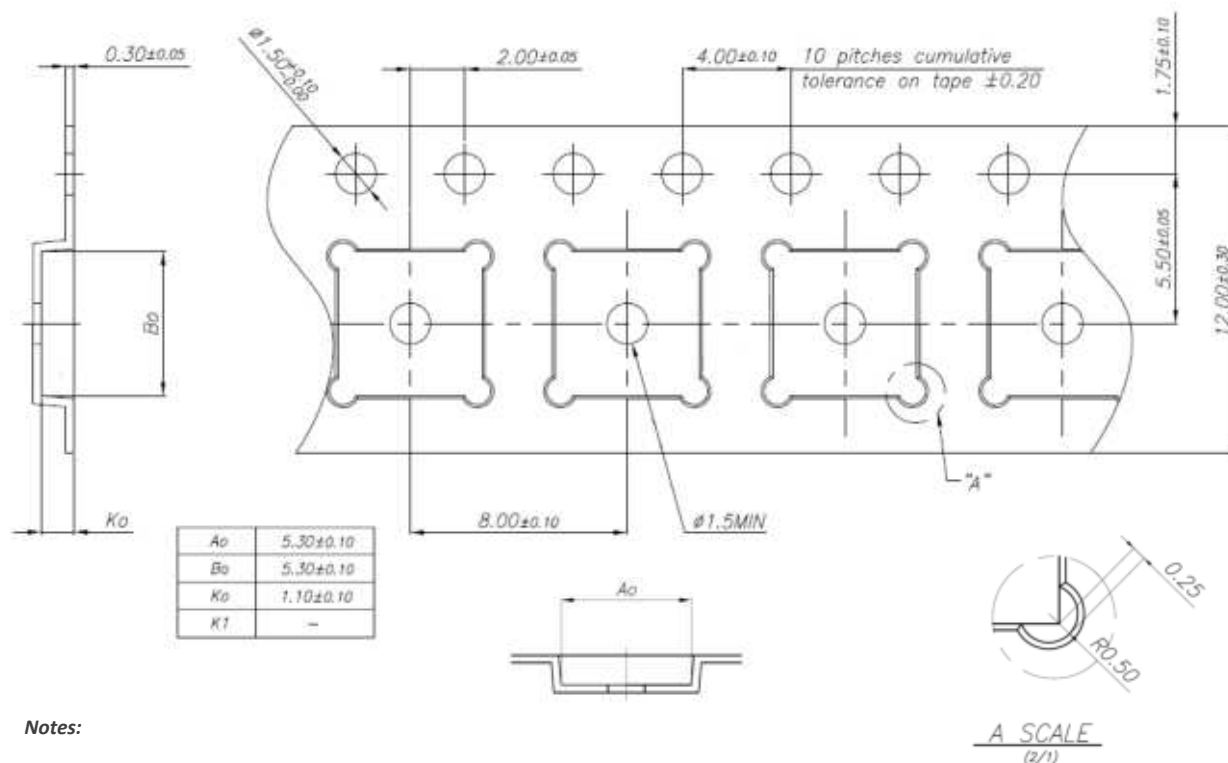
Figure 84. Tape & Reel
