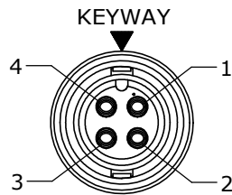
FACE VIEW P/N: CA63804SXXX90
