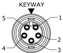
FACE VIEW P/N: CA63805SXXX90
