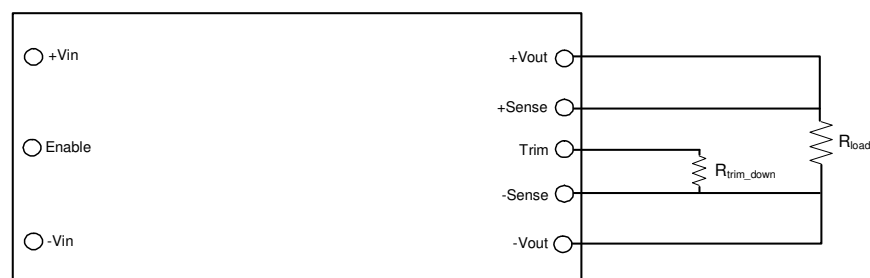
Figure 14. Trim DOWN circuit configuration
