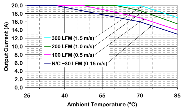
Figure 4. Output Current Derating vs Ambient Temp (converter mounted vertically with air flowing from pin 3 to pin 1, Vin = 48 Volts, with baseplate)
