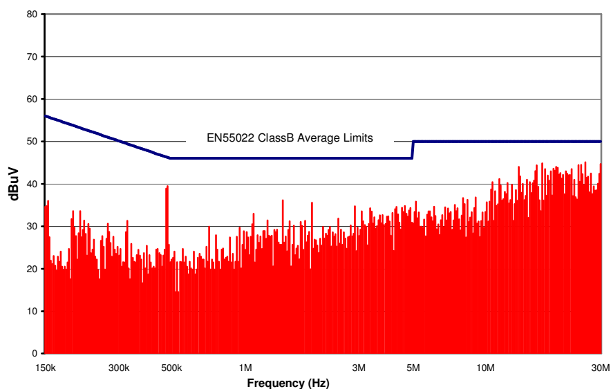
Figure 16. CPT20A48 Conducted Emissions using above specified input filter. Vin = 48V, Full Resistive Load
