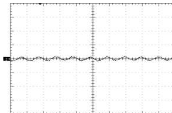
Figure 6. Input Reflected Ripple Current (10 mA/div) time scale - 2uS/div. Vin=Vin_nom, full resistive (see Fig 11)
