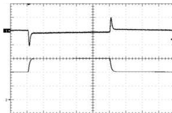
Figure 10. Load Transient Response (100mV/div), di/dt=0.1A/uS, 50% - 75% - 50% of full load, time scale: 200uS/div Ch1=100mV/div, Ch2=5A/div
