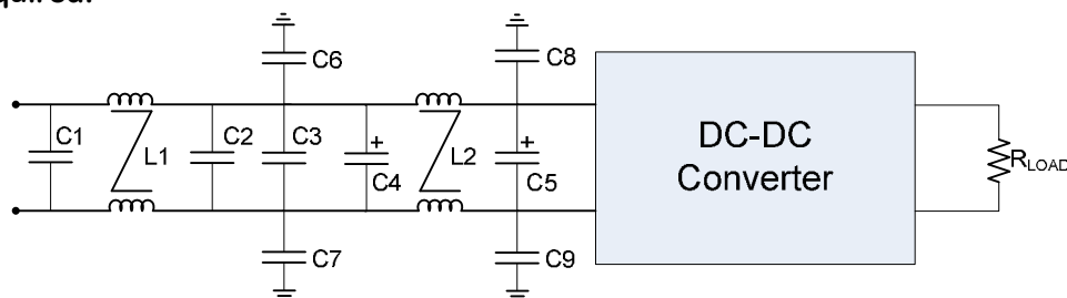
Figure 15. EMI Filter
