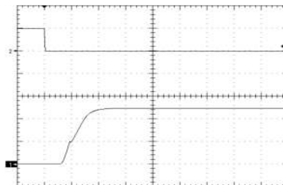
Figure 8. Startup Waveform via Enable Pin, time scale 10mS/div. Vin=Vin_nom, full resistive load + 10000uF, Ch1=2V/div, Ch2=5V/div
