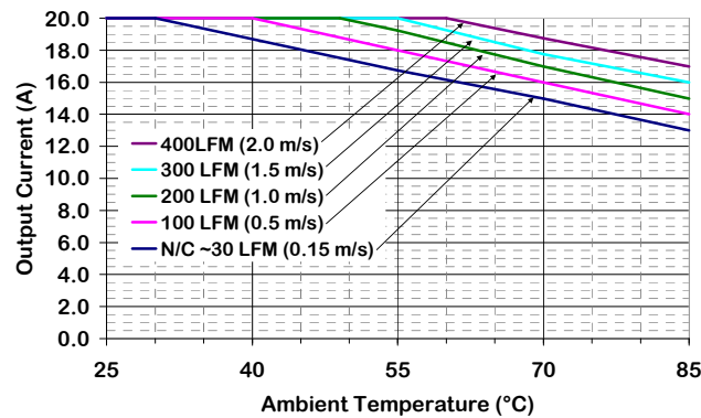
Figure 3. Output Current Derating vs Ambient Temp (converter mounted vertically with air flowing from pin 3 to pin 1, Vin = 48 Volts, without baseplate)
