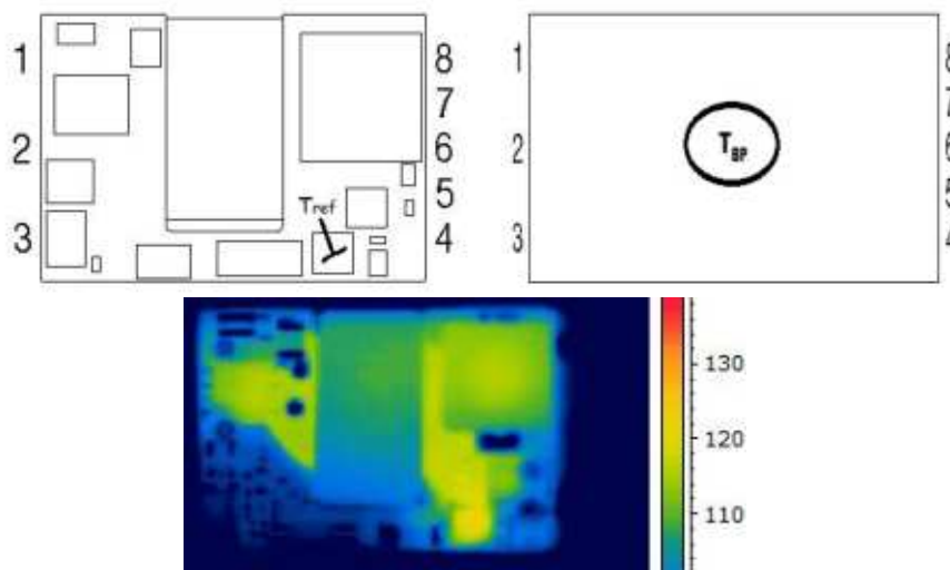
Thermal Image of Module - Vin=48V, Full Load @ 55C, 300LFM
