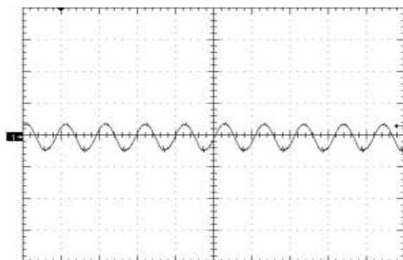
Figure 5. Output Voltage Ripple (50mV/div), time scale – 2uS/div. Vin=Vin_nom, full resistive Cout=1uF ceramic + 10uF ceramic (see Fig 12)
