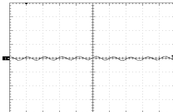
Figure 6. Input Reflected Ripple Current (10mA/div) time scale - 2μS/div. Vin=Vin_nom, full load
