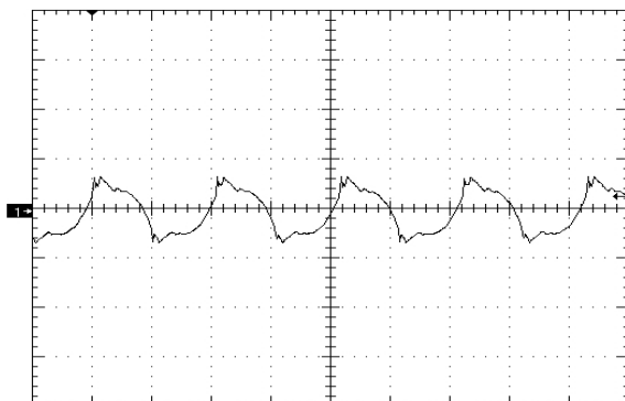
Figure 5. Output Voltage Ripple (50mV/div), time scale – 1μS/div. Vin=Vin_nom, full load Cout=1μF ceramic + 10μF Tantalum (see Fig 12)
