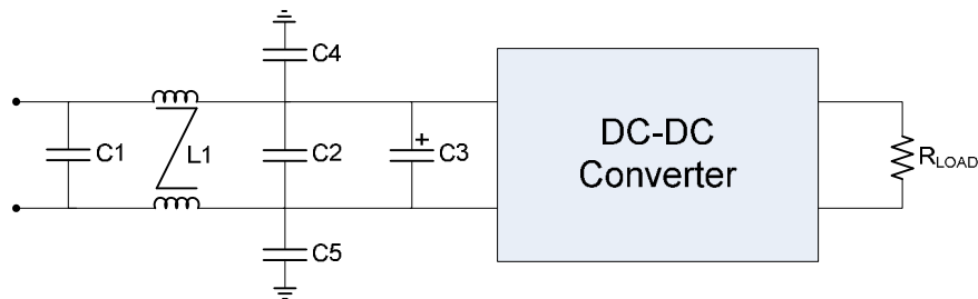
Figure 16. EMI Filter
