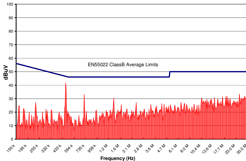
Figure 17. CPT20F48 Conducted Emissions using above specified input filter. Vin = 48V, Full Resistive Load
