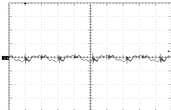
Figure 7. Output Voltage Ripple (20mV/div), time scale – 1μS/div. Vin=Vin_nom, full load Cout=1μF ceramic + 47μF ceramic (see Fig 13)
