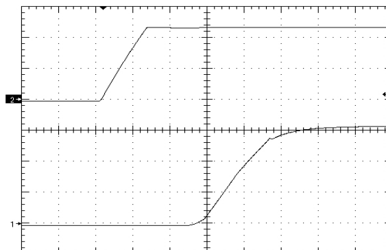
Figure 8. Startup Waveform (1V/div) via Vin, time scale 4mS/div. Vin=Vin_nom, full resistive load + 10000μF.
