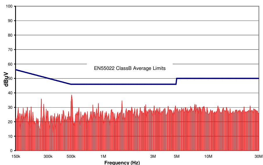
Figure 18. CPT3B48 Conducted Emissions using above specified input filter. Vin = 48V, Full Resistive Load
