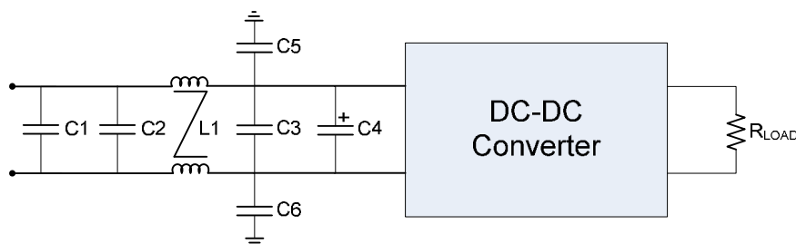
Figure 17. EMI Filter
