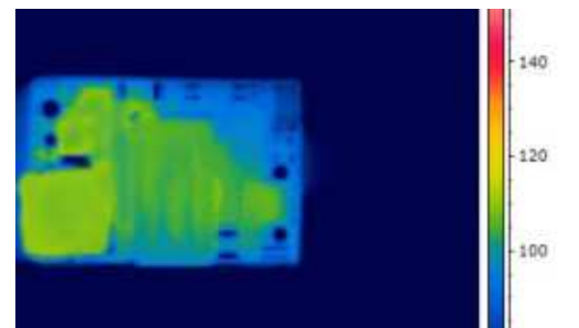
Figure 4. Thermal Image of CPT3B48 (2.5A output, 85C Ambient, natural convection, Vin = 48V, airflow from pin 3 to pin 1, T_{max} = 111^{\circ}\text{C} )
