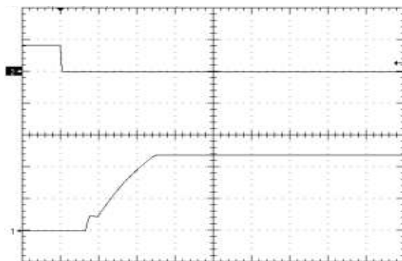
Figure 9. Startup Waveform via Enable Pin, time scale 10mS/div. Vin=Vin_nom, full load Ch1=5V/div, Ch2=5V/div
