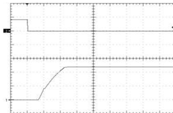
Figure 10. Startup Waveform via Enable Pin, time scale 10mS/div. Vin=Vin_nom, full resistive load + 820uF. Ch1=5V/div, Ch2=5V/div
