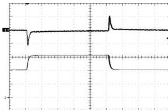
Figure 10. Load Transient Response (100mV/div), di/dt=0.1A/uS, 50% - 75% - 50% of full load, time scale: 200uS/div
