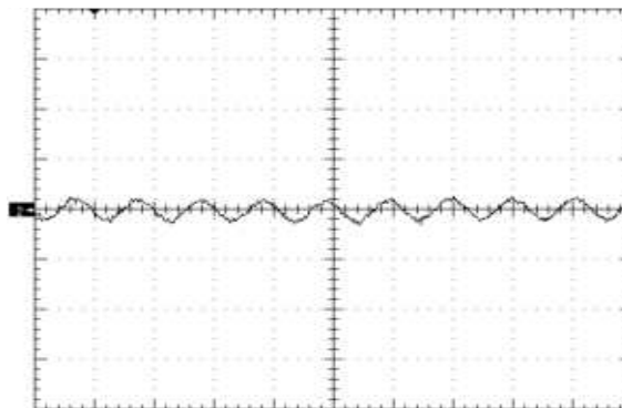
Figure 6. Input Reflected Ripple Current (10mA/div) time scale - 2uS/div. Vin=Vin_nom, full resistive.
