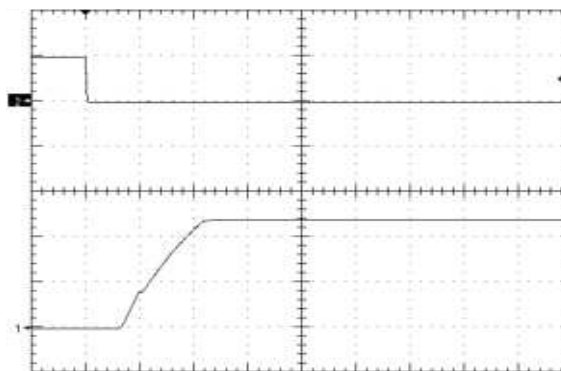
Figure 8. Startup Waveform via Enable Pin, time scale 10mS/div. Vin=Vin_nom, full res. load + 4700uF, negative enbl, Ch1=5V/div, Ch2=5V/div
