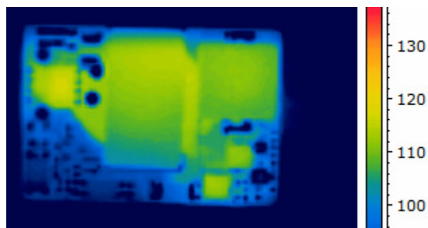
Figure 4. Thermal Image of CPT8B48 3A output, 55C Ambient, 200lfm airflow, Vin = 48V, airflow from pin 3 to pin 1, T_{max} = 116^{\circ}\text{C}
