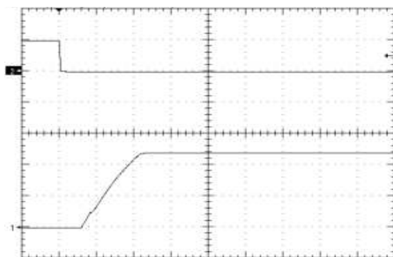
Figure 7. Startup Waveform via Enable Pin, time scale 10mS/div. Vin=Vin_nom, full load Ch1=5V/div, Ch2=5V/div
