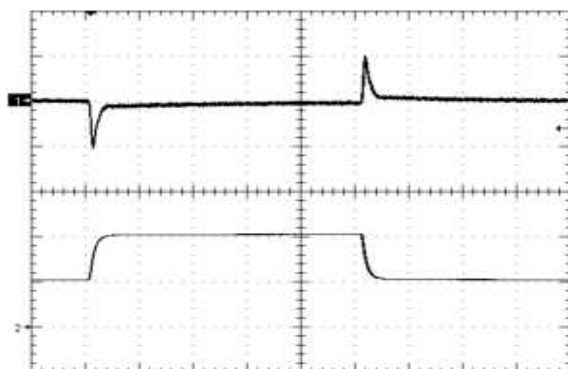
Figure 9. Load Transient Response (100mV/div), di/dt=0.1A/uS, 50% - 25% - 50% of full load, time scale: 200uS/div
