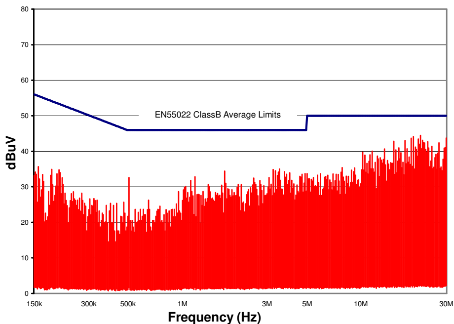
Figure 16. CPT8B48 Conducted Emissions using above specified input filter, Vin = 48V, Full Resistive Load
