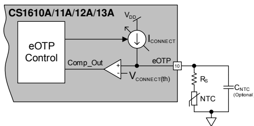
Figure 17. eOTP Functional Diagram
