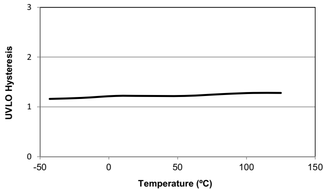
Figure 3. UVLO Characteristics
