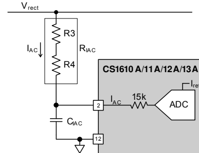
Figure 13. IAC Input Pin Model
