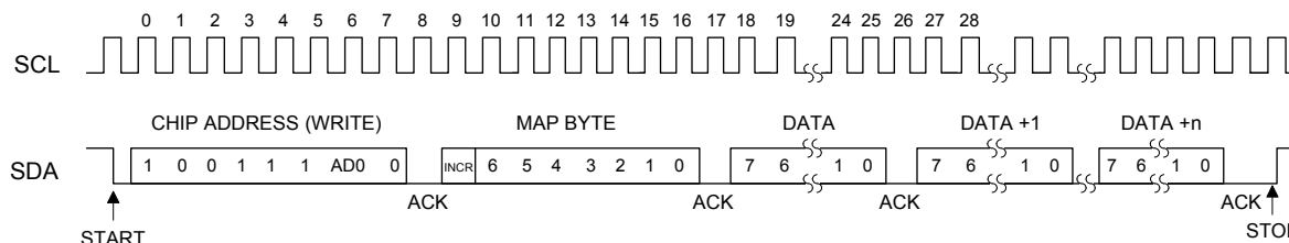
Figure 22. Control Port Timing, I²C Write
