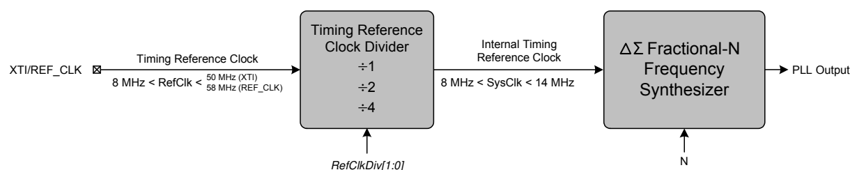
Figure 8. Internal Timing Reference Clock Divider
