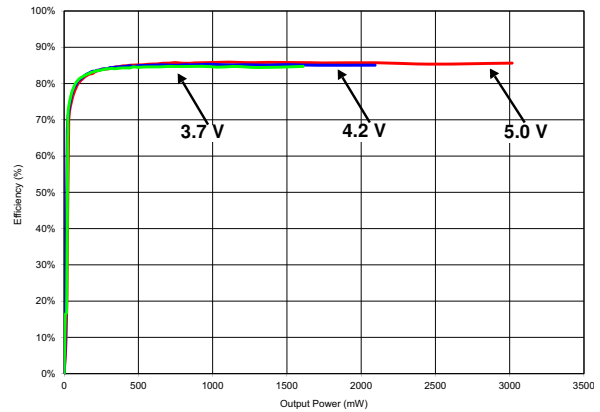
Figure 53. Efficiency vs. Output Power - FHD Mode R_L = 4 \Omega + 33 \mu\text{H}
