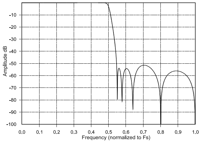
Figure 9. Single-Speed Stopband Rejection
