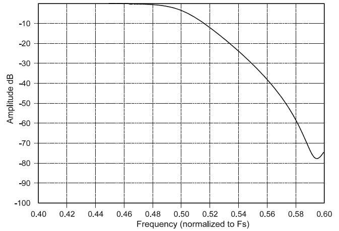
Figure 14. Double-Speed Transition Band
