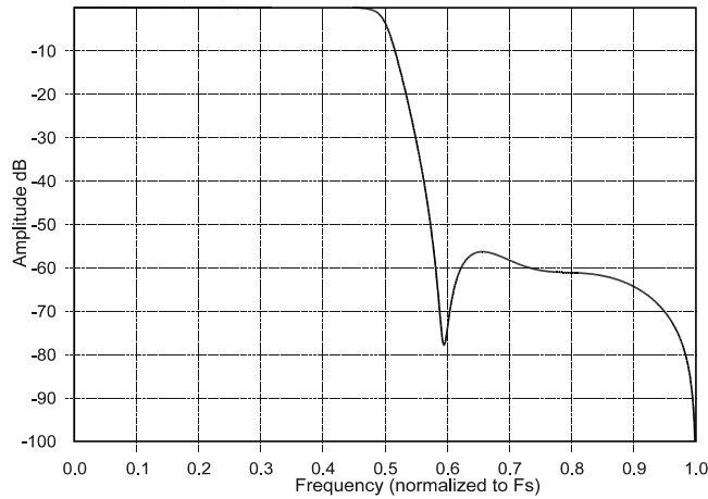
Figure 13. Double-Speed Stopband Rejection
