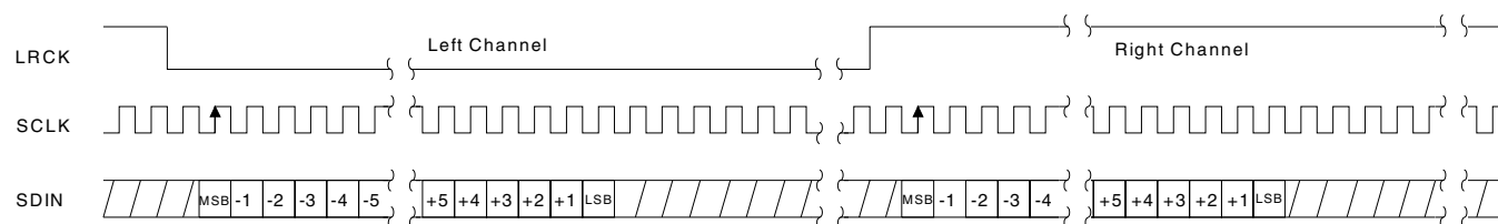
Figure 2. I²S Data
