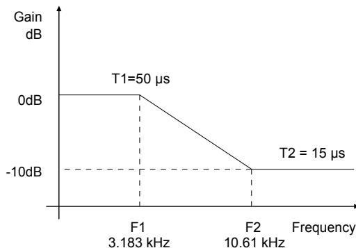
Figure 5. De-Emphasis Curve
