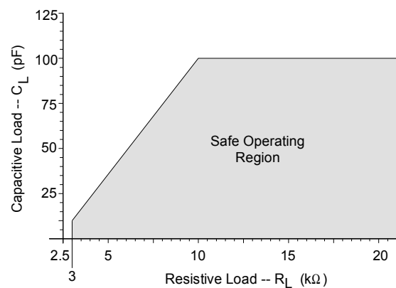
Figure 10. Maximum Loading
