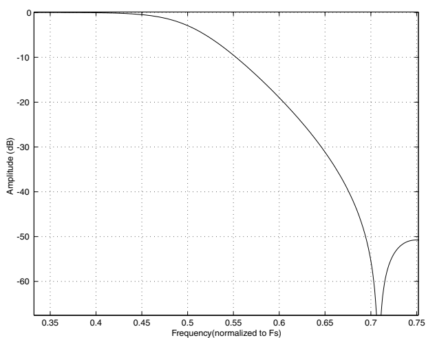
Figure 21. Quad-Speed Transition Band
