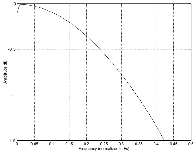
Figure 23. Quad-Speed Passband Ripple
