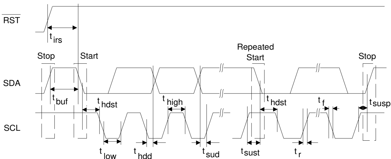
Figure 4. Control Port Timing - I 2 C Format
