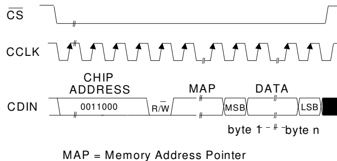
Figure 23. Control Port Timing, SPI Mode
