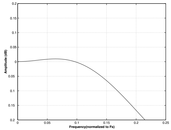
Figure 39. Quad-Speed (fast) Passband Ripple
