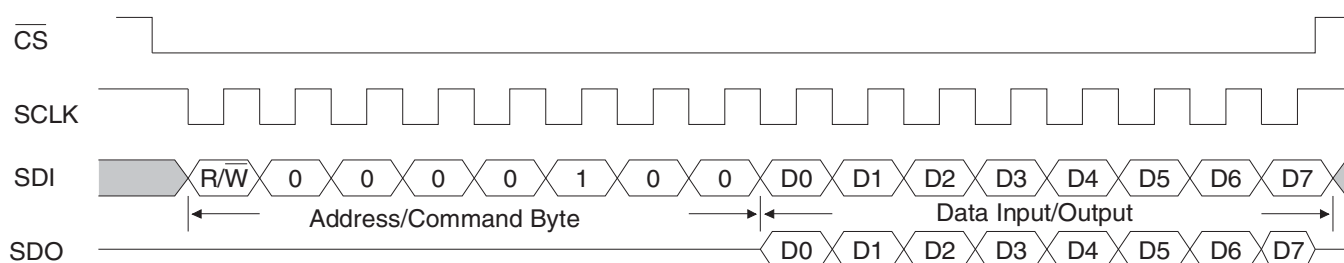
Figure 13. Input/Output Timing
