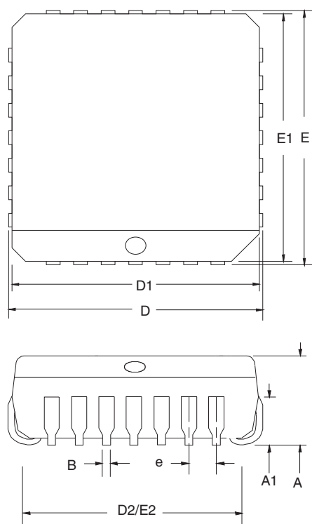
28-pin PLCC
