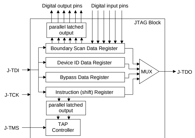
Figure 23. JTAG Circuitry Block Diagram
