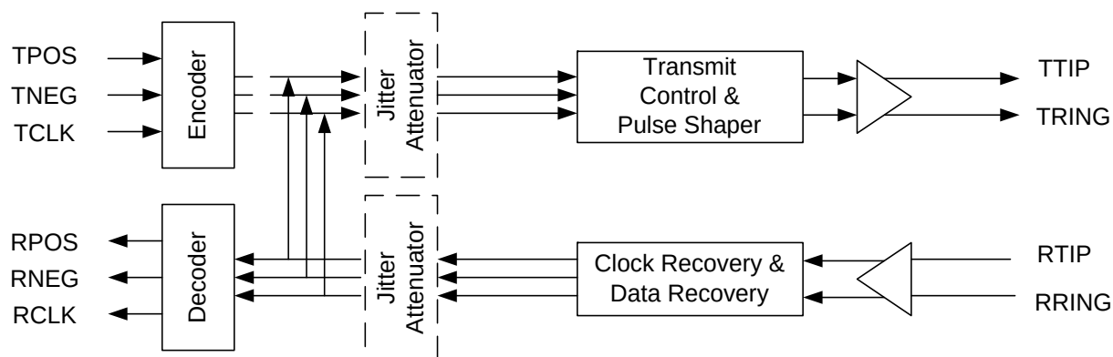
Figure 12. Remote Loopback Block Diagram
