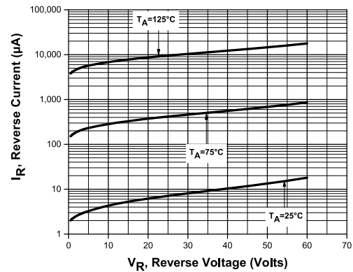
Leakage Current for CSHDD16-60C
