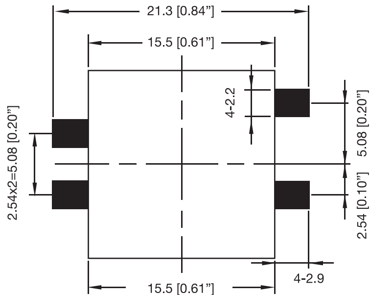
Reverse Mount
