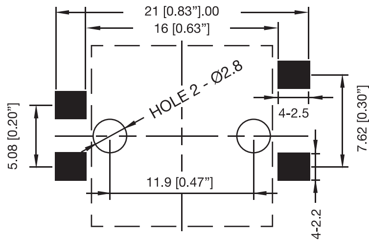
Top Mount
